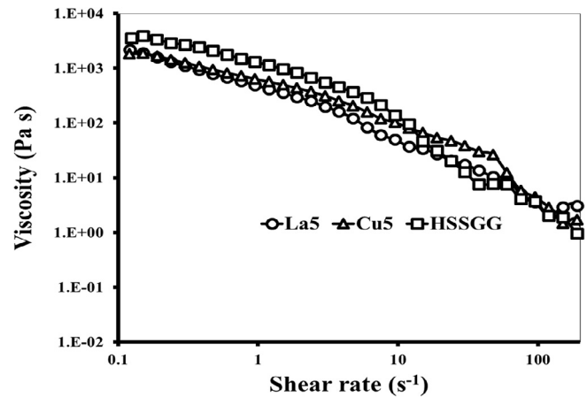
Fig. 4. Comparison of the flow properties of suspensions prepared from HSSGG, Cu5 and La5 glass powders.
