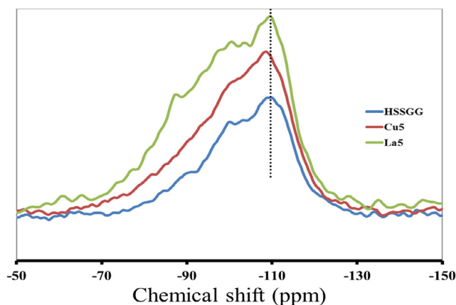
Fig. 2. ^{29}\text{Si} NMR for HSSGG (blue line), Cu5 (brown line) and La (green line) doped glasses. (For interpretation of the references to colour in this figure legend, the reader is referred to the web version of this article.)
