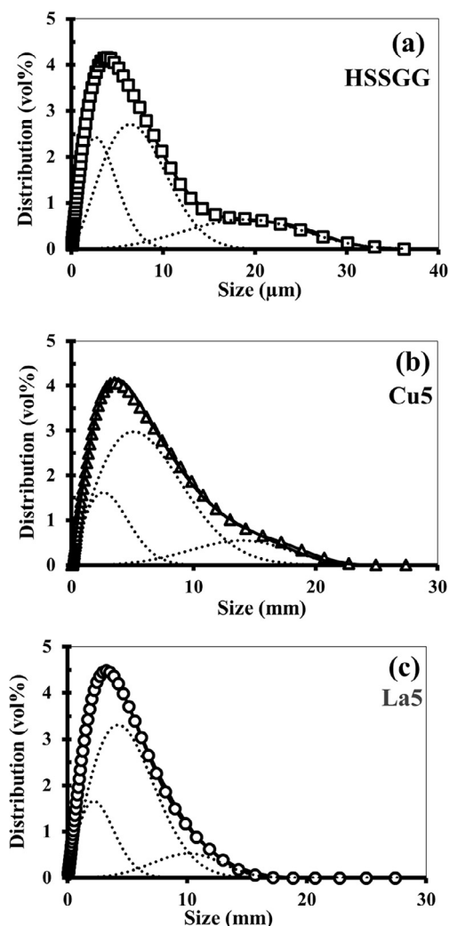
Fig. 1. The ion doping effects on the particles size distributions of the wet-milled glass powders: (a) HSSGG, (b) Cu5 and (c) La5.
