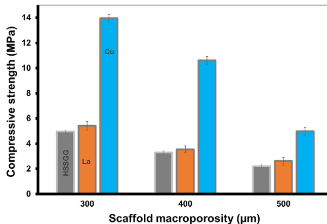
Fig. 7. Compressive strength of the scaffolds, fabricated from HSSGG, Cu5 and La5 glasses, with different macro-pore sizes (300, 400 and 500 \mu\text{m} ) sintered at 800 ^{\circ}\text{C} .
