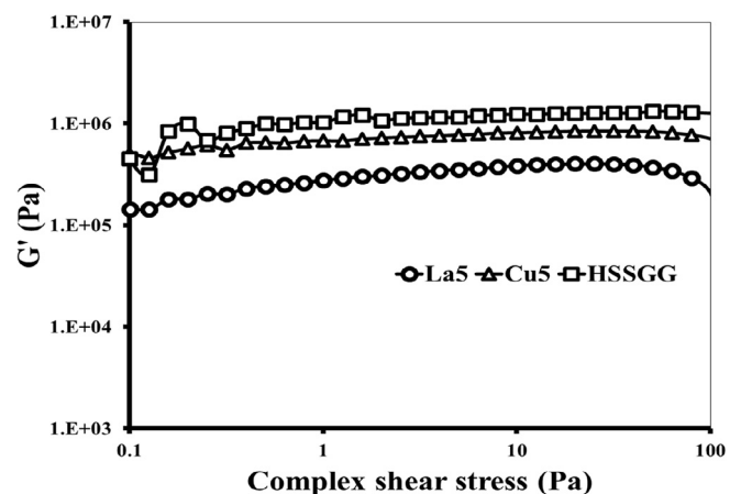
Fig. 5. Elastic modulus ( \hat{G} ) and extent of LVR as a function of complex shear stress of suspensions/pastes prepared from HSSGG, Cu5 and La5 glass powders.
