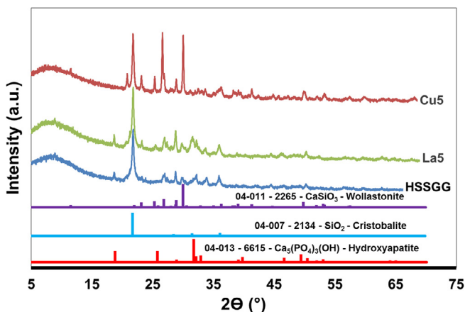
Fig. 3. Comparison of the XRD patterns of parent HSSGG composition with La5 and Cu5-containing samples.
