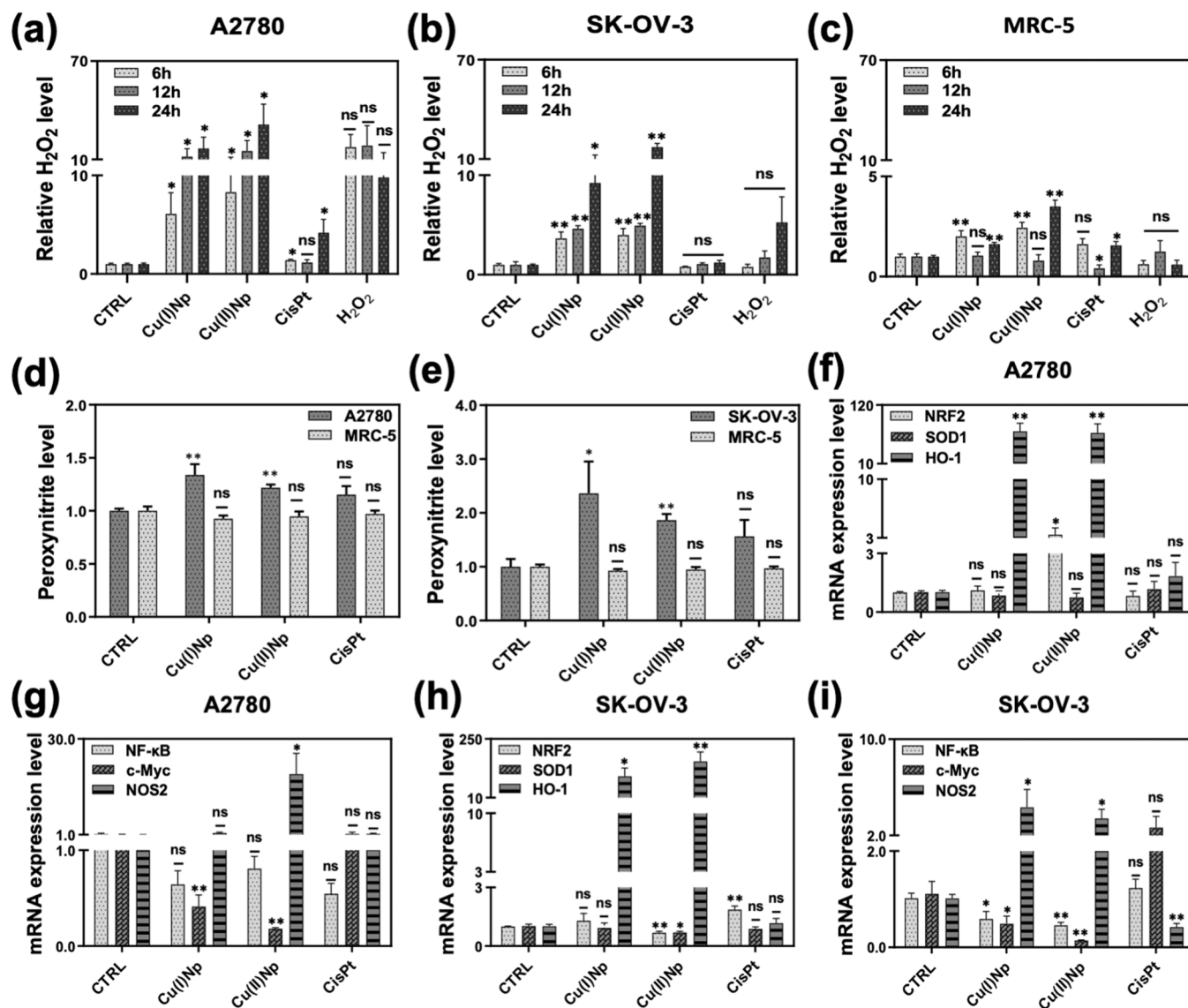
Fig. 5. CuNP generates multiple ROS in cancer cell lines. a-c , Relative H_2O_2 level measurement. a , A2780, b , SK-OV-3, c , MRC-5. d-e , Relative ONOO^- level measurement. A2780, S-KO-V3, and MRC-5 f-i , qPCR analyses of selected genes. Bar graphs represent real-time RT-PCR analyses for mRNA expression of A2780 and SK-OV-3 cell lines after 24 h of CuNP treatment. f , h , NRF2, SOD1, HO-1, g , i , NF- \kappa B, c-Myc, NOS2. Cells were incubated with CuNP (10 \mu g/ml), and CisPt (3 \mu g/ml; 10 \mu M) for 24 h; error bars indicate SEM. Data shown are two independent experiments of three replicates.
