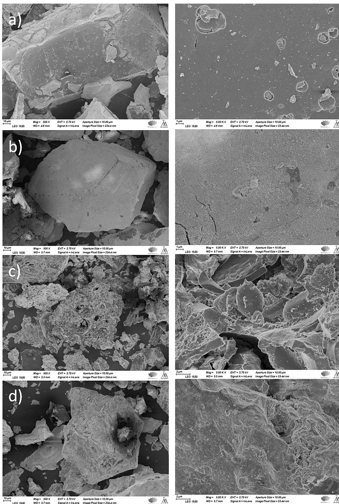
Fig. 5. The SEM images of (a) \text{NiAl}/\text{A}_\text{T} , (b) \text{NiAlP}/\text{A}_\text{T} , (c) \text{NiAlP}/\text{A}_\text{W} , and (d) \text{NiAlP}/\text{A}_\text{B} catalysts, with 500X and 5.00 K X magnifications.
