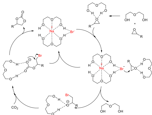
Figure 2. Proposed mechanism for the co-catalytic effect of DEG. Top, mid: the activation of NaBr; top-to-bottom, right: hydrogen bond donor assistance to the epoxide ring cleavage.
