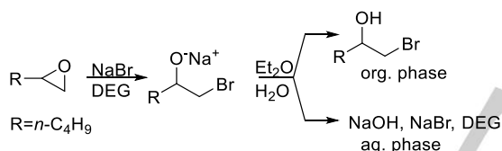
Scheme 6. Hydrolysis of the alcoholate precursor of bromohydrin
