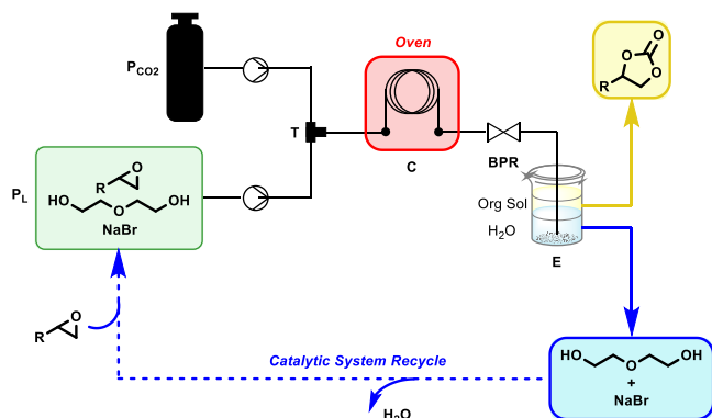
Figure 3. CF apparatus used for CF CO 2 insertion into epoxides
