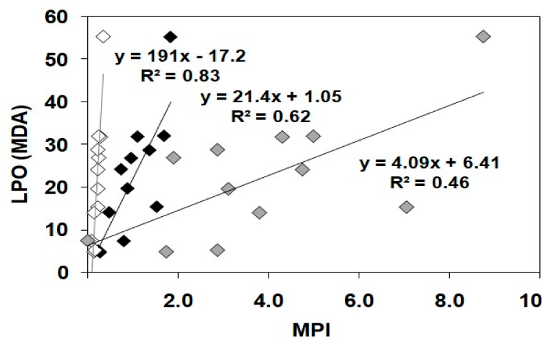
Figure 3. The plot of correlation between MPI and LPO levels for U. laetevirens collected in the three VL sites. Solid white squares □ indicated MPI/concentration of Hg alone, solid black squares ■ indicated MPI calculated for As, Hg and Pb together, and solid gray squares ■ indicated the MPI calculated for the overall metals.
