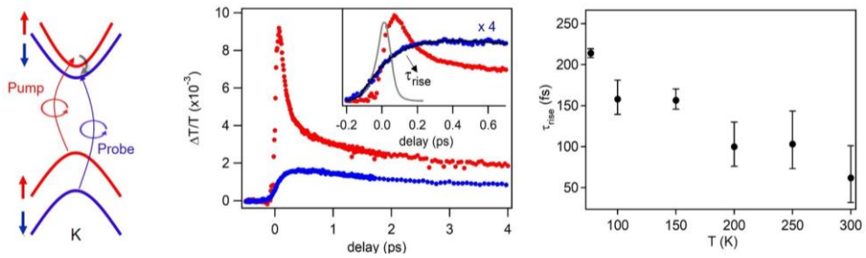
Fig. 1. (Left panel) Sketch of the band structure of 1L-WS 2 around the K point of the Brillouin zone. The pump and probe pulses have the same circular polarization. The pump is resonant with the A exciton while the probe is resonant with either the A (degenerate configuration) or B exciton (non-degenerate configuration). Only the non-degenerate configuration is sketched for sake of clarity. Only excitons in K point are excited because of the valley dependent optical selection rules for circular polarization. The intravalley scattering process (grey arrow) from upper to lower CB state causes the reduction of the absorption of the probe beam by Pauli blocking and results in a delayed formation of the bleaching signal around the B exciton. (Central panel) The red and blue curves are the \Delta T/T signal measured in 1L-WS 2 at 77K around the A and B excitonic transitions, following excitation of the A transition. For degenerate pump and probe energies, the build-up dynamics is pulse-width limited, while the non-degenerate configuration displays a delayed formation. In the inset, \Delta T/T around the B exciton peak is multiplied by 4 to highlight the finite build up time. The grey line is the cross correlation function between the pump and probe pulses. (Right panel) Temperature dependence of the B exciton rise time \tau_{\text{rise}} .
