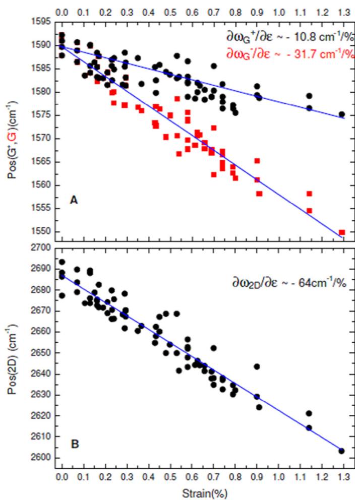
Figure IX.41. Change in \text{Pos}(G) and \text{Pos}(2D) with increasing tensile, uniaxial strain. Adapted from [1529], copyright American Chemical Society.
