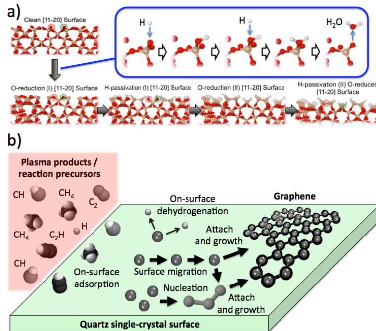
Figure V.35. (a) Side view of the different DFT-computed steps along the reduction process of the [11-20] quartz surface (adapted from [774], © IOP Publishing Ltd): starting from the clean hydroxylated surface [976] across subsequent protonation barrierless steps and detachment of \text{H}_2\text{O} molecules (see inset), which lead to slight surface reconstructions, and H-passivation of the surface. (b) sketch corresponding to the coexisting processes leading to the growth of graphene on a quartz single-crystal surface from the different plasma products by PECVD: adsorption, decomposition and dehydrogenation of the reaction precursors, toward graphene nucleation and formation.
