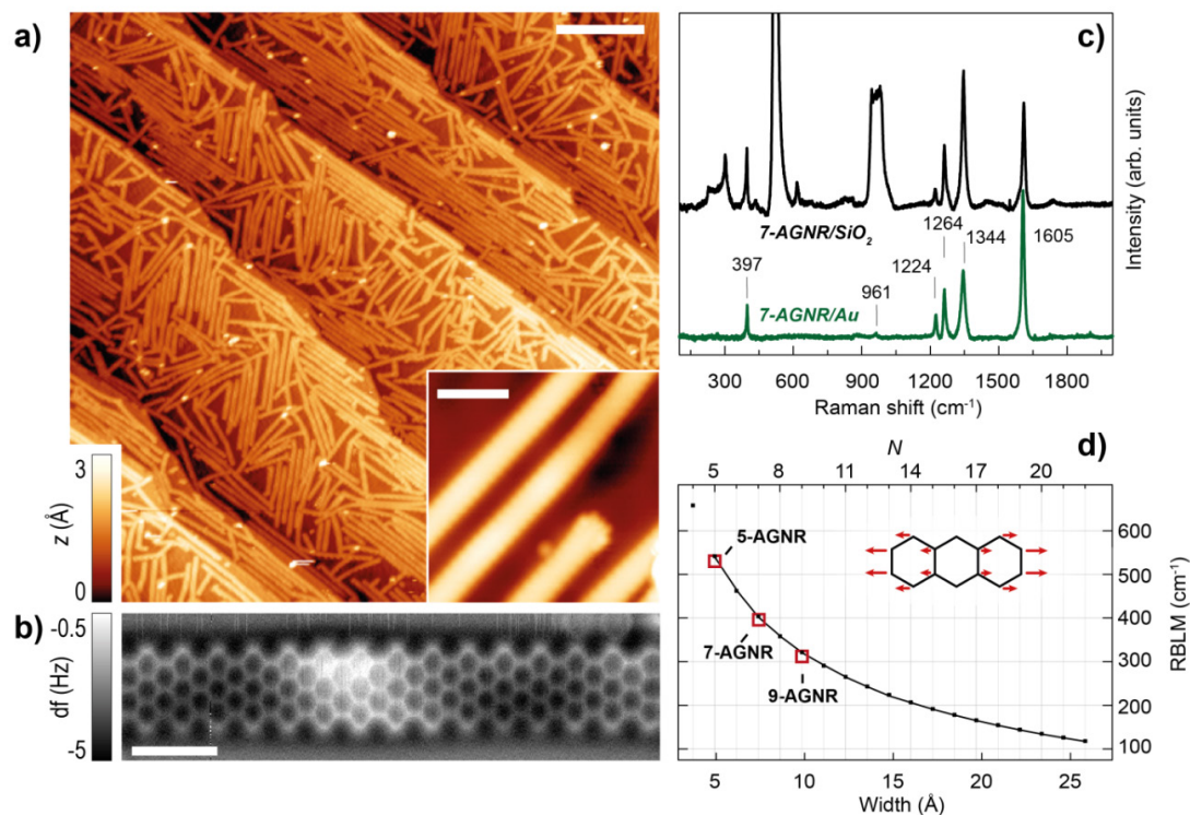
Figure 1.4. Characterization of 7-AGNRs on their growth substrate and after substrate transfer. (a) Large-scale STM topography image (bias: -0.5 V; current: 5 pA; T : 4.5 K; scale bar: 30 nm) showing high coverage 7-AGNRs on Au(111). Inset: small-scale STM image (bias: 0.1 V; current: 30 pA; scale bar: 3 nm). The apparent height of individual 7-AGNRs is 0.19 nm. (b) Constant-height nc-AFM frequency shift image (bias: 2 mV; oscillation amplitude: 0.3 Å; T : 4.5 K; scale bar: 1 nm) taken with a CO-functionalized tip. (c) Raman spectra of 7-AGNR on Au(111) recorded under ambient conditions after synthesis (green curve) with indicated peak positions of the main modes, and after transfer to Si/SiO 2 (black curve; laser 532 nm, power of 2 mW, three scans of 20 s). (d) RBLM peak position for 5-AGNRs, 7-AGNRs and 9-AGNRs (red markers), together with predicted width-dependent RBLM wavenumbers for AGNRs [65].
