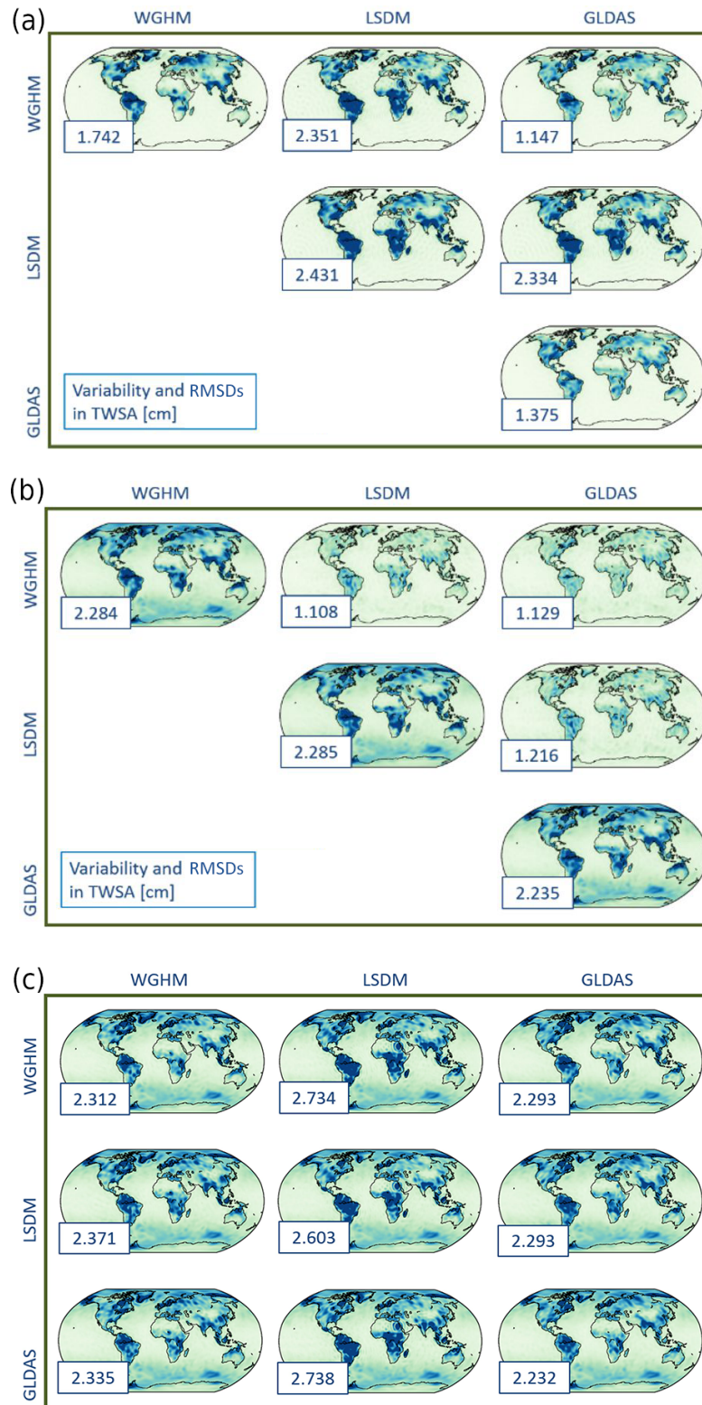
Figure 1. (a) Global average daily water mass variability (main diagonal) and root mean square differences (RMSDs) (off-diagonal) between the hydrological models used, expressed as TWASs (2003–2014, secular and annual variations removed). (b) Global average daily variability (main diagonal) and RMSDs (off-diagonal) of the derived daily ITSG-Grace2014 solutions, expressed as TWASs (2003–2014, secular and annual variations removed). (c) Global RMSDs in cm between the daily ITSG-Grace2014 solutions (rows) and the hydrological models used (columns), expressed as TWASs (2003–2014, secular and annual variations removed).
