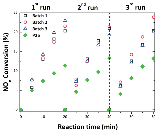
Fig. 5 Photocatalytic \text{NO}_x abatement test in triplicate of the three K7000 batches, and P25 as comparison, using the white LED lamp.
