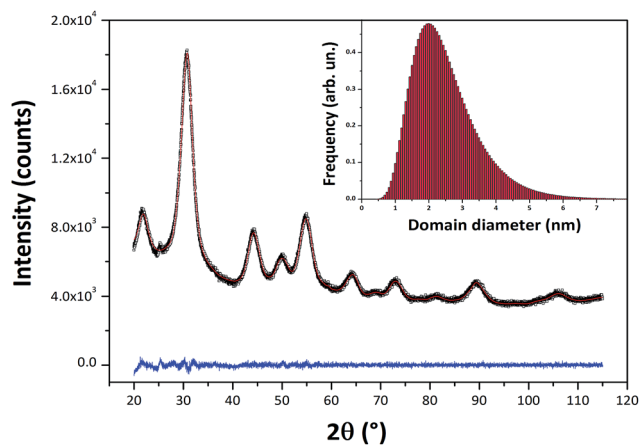
Fig. 2 Graphic output of the WPPM modelling of the SrHfO 3 sample. The black open squares represent the observed pattern, the continuous red line represents the calculated pattern, and the difference curve between observed and calculated profiles is the blue continuous line plotted below. In the inset is reported the crystalline domain size distribution of SrHfO 3 .
