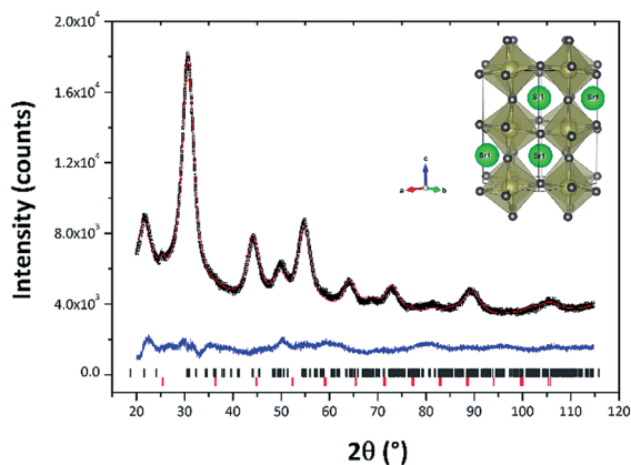
Fig. 1 Graphic output of the Rietveld refinement of the SrHfO 3 sample. The black open squares represent the observed pattern, the continuous red line represents the calculated pattern, and the difference curve between observed and calculated profiles is the blue continuous line plotted below. The positions of reflections are indicated by the small vertical bars (dark grey = SrHfO 3 , red = Sr). In the inset is reported a 3D rendering of the SrHfO 3 crystal structure (space group, Pbnm ). The small dark grey spheres represent oxygen, the larger dark green spheres are hafnium (coordination VI), whilst the largest, light green spheres are strontium (coordination X). Octahedral tilting of the perovskite ( a − b + a − , using the Glazer's notation, as obtained using SPuDS software) can be appreciated from the 3D rendering.
