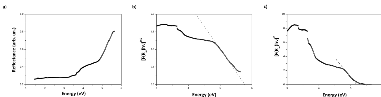
Fig. 5 (a) Diffuse reflectance spectrum of SrHfO 3 – reflectance versus energy. (b) and (c) show the Kubelka–Munk elaborations for the same sample. In (b), the dotted line represents the x -axis intercept of the line tangent to the inflection point, e.g. its apparent optical E_g (5.78 eV), calculated with the Tauc procedure, and assuming the transition to be indirectly allowed (power coefficient \gamma = 1/2 ). In (c), the dashed line represents the x -axis intercept of the line tangent to the inflection point, e.g. its apparent optical E_g (5.20 eV), calculated with the Tauc procedure, and assuming the transition to be directly allowed (power coefficient \gamma = 2 ).
