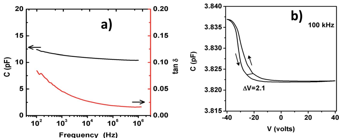
Fig. 7 (a) Frequency and (b) bias voltage dependence of capacitance.
