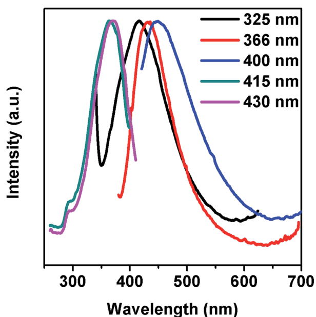
Fig. 6 Room temperature emission spectra of pure SrHfO 3 excited at 325, 366, 400, 415 and 430 nm.
