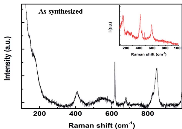
Fig. 4 Raman spectrum of as-synthesised SrHfO 3 nanoparticles, and in the inset, those annealed at 800 °C.
