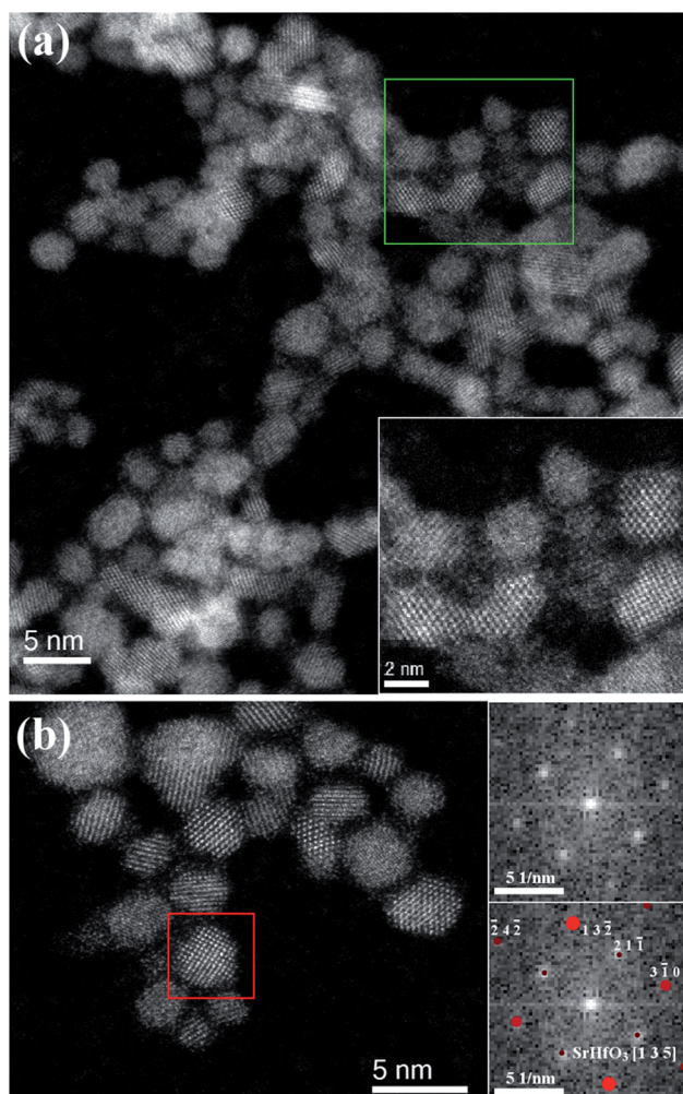
Fig. 3 HRSTEM-HAADF micrographs of as-synthesised SrHfO 3 NPs. The inset in (a) shows a magnified view of the area demarcated by the green square. The insets in (b) display the FFT pattern obtained from a single NP (red square) (top) and the superposition with the simulated diffraction pattern obtained with the SrHfO 3 Pbnm type perovskite structural data described in Table 1 in the [1 3 5] zone axis (bottom).
