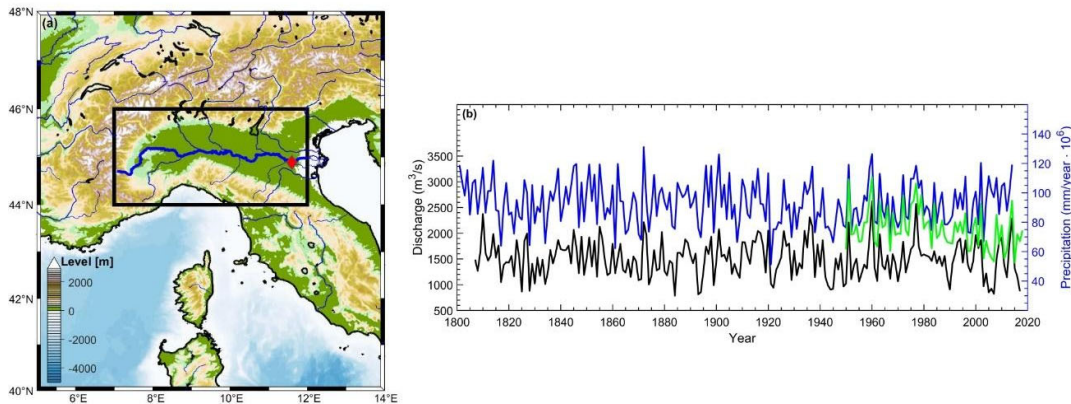
Figure 1. (a) Po River basin and location of the Pontelagoscuro gauge station ( 44^{\circ} 53' 19.34'' N, 11^{\circ} 36' 29.60'' E; red diamond). This map was obtained with MATLAB using the m_map package [19] and the GSHHG dataset for coastlines [20–22] and the ETOPO one [23] for elevation and bathymetry. The black rectangle represents the area over which total annual precipitations were evaluated over the Po plain ( 44 – 46^{\circ} N, 7 – 12^{\circ} E). (b) Comparison between annual Po discharges (black curve) and total annual precipitation (blue curve) over the Po basin using data from the HISTALP dataset. From the year 1950 onward, precipitation data from the E-OBS dataset (green curve in (b)) are also considered.
