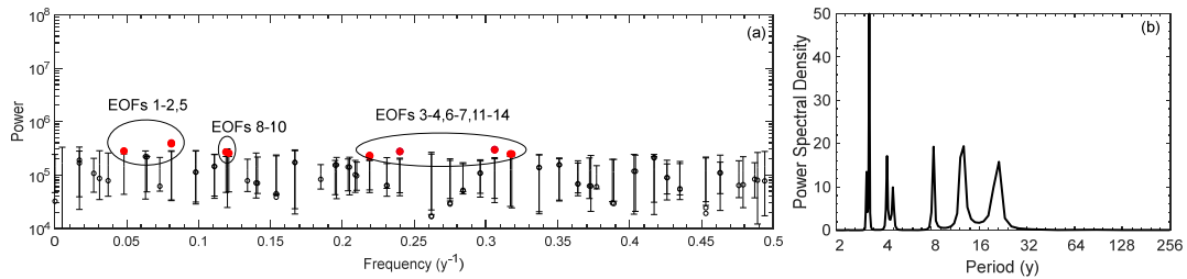
Figure 3. Spectral properties of the Po River discharge series. (a) Monte Carlo-SSA test performed using EOFs 1–14 and AR(1) as the null hypothesis model (window width W = 80 y and Monte Carlo ensemble size 10,000). The red dots mark the eigenvalues corresponding to the empirical orthogonal functions (EOFs) included in the null hypothesis. No excursions occur outside the 99% limits, indicating that the series is well explained by this model. The periods associated with the reconstructed components (RCs) are: \sim 12 y (RCs 1–2,5), \sim 8 y (RCs 8–10) and \sim 3 y (3–4, 6–7, 11–14). (b) Power spectrum obtained performing the spectral analysis of the sum of all the significant components of the Po discharge series, performed using the maximum entropy method (order 20, see [35] and references therein).
