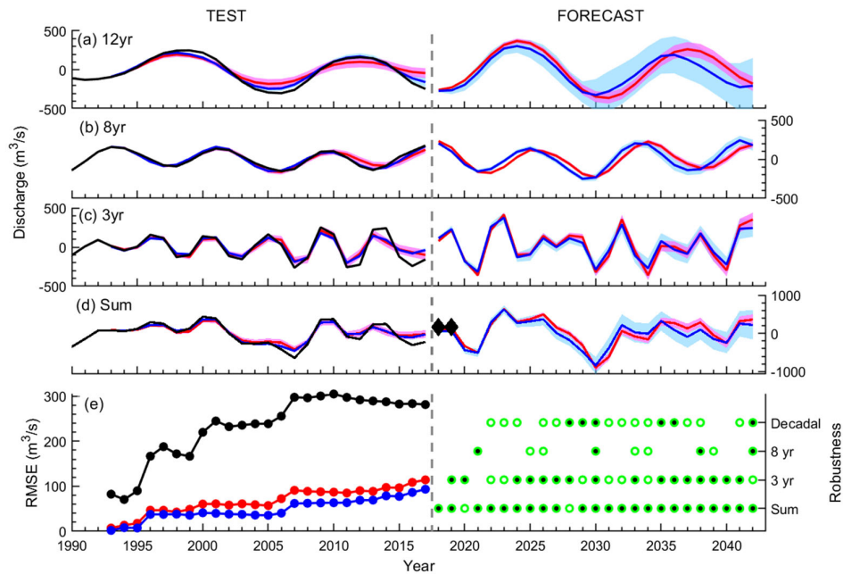
Figure 4. (a–d) Prediction (left column) and forecast (right column) results for the three components of the Po River discharges over the test (1993–2017) and the forecast (2018–2042) sections. In black, the RCs reconstructed by SSA are plotted, while in red the predictions obtained by the AR method and in blue those obtained by the NN method are shown with the associated error bands. All components are represented as zero-mean. Black diamonds in (d) represent the values of the SSA components obtained analyzing the record including the 2018–2019 period. This SSA analysis was applied using a window width w = 80 y and the significant components extracted are RCs 1–13,15–16. (e) Left column: progressive RMSE as a function of lead time evaluated for both the AR and NN methods (dotted red and blue curves, respectively) and for the persistence hypothesis (dotted black curve). The RMSE is evaluated between the denoised discharge time series (black curve in (d)) and the corresponding predictions. Right column: results of the compatibility test performed between the AR and NN forecasts for each time step. Black dots indicate when the predictions are robust, namely when their difference is compatible with 0 (in the 1\sigma range). Empty green dots indicate when the difference is null in the 2\sigma range.
