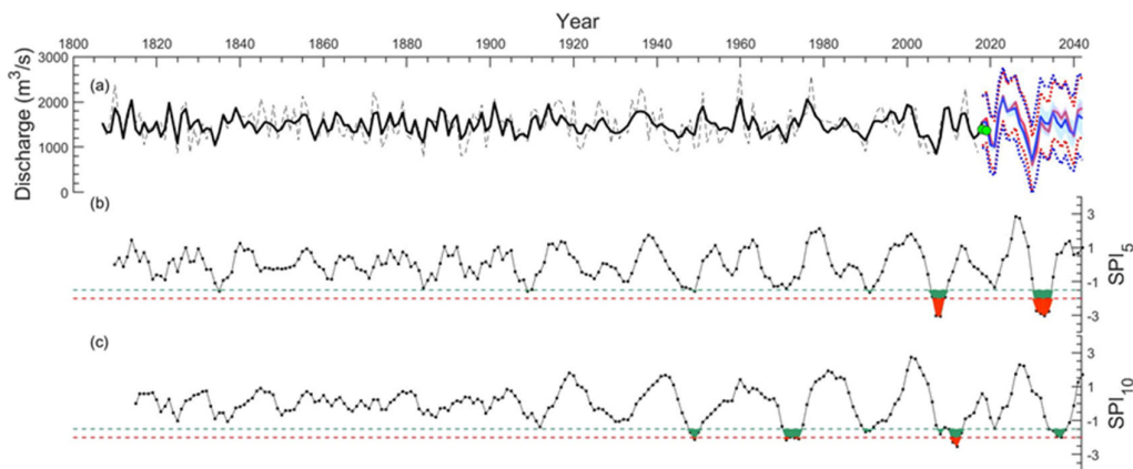
Figure 5. Standardized precipitation index (SPI) time series calculated for Po River discharge denoised series and the forecasted time period 2018–2042. (a) Po River discharges (dotted black curve) and corresponding denoised series (black curve) with the associated forecast obtained using the AR model (red curve) and the feed-forward neural network (FFNN) method (blue curve). Dotted blue and red curves represent the total uncertainty associated with the forecasts, considering also the contribution of the residuals. Green dots represent raw annual average discharge data for the period 2018–2019. (b–c) Five-year and ten-year SPI time series. The horizontal lines individuate the thresholds for the categories of severity by [38], namely moderate (SPI = -1, green line) and extreme (SPI = -2, red line) droughts. The colored areas indicate periods when the Po River basin experienced moderate (green areas) and extreme (red areas) droughts.
