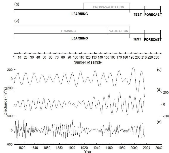
Figure 2. (a,b) Schematic diagram of the sections in which the input data series were divided according to the prediction method selected. For both autoregressive (AR) and neural network (NN) models, the length of the learning, test and forecast sections are the same. Nevertheless, while the AR algorithm uses all the available data to evaluate the coefficients of the autoregressive model (a), the NN method requires that the learning section be further divided into training and validation subsections (b), as described in the text. Both methods were applied to evaluate the hindcasts over the test section in order to compare the predictions to the data included in the last portion of the time series. Finally, the forecasts for the next 25 years are evaluated for the forecast section. Uncertainties associated with AR forecasts were obtained performing 25-year predictions over different portions of this time interval (cross-validation subsection) and then evaluating the RMSE between the predicted and original data as a function of the lead time. (c–e) Significant oscillatory components in the Po
