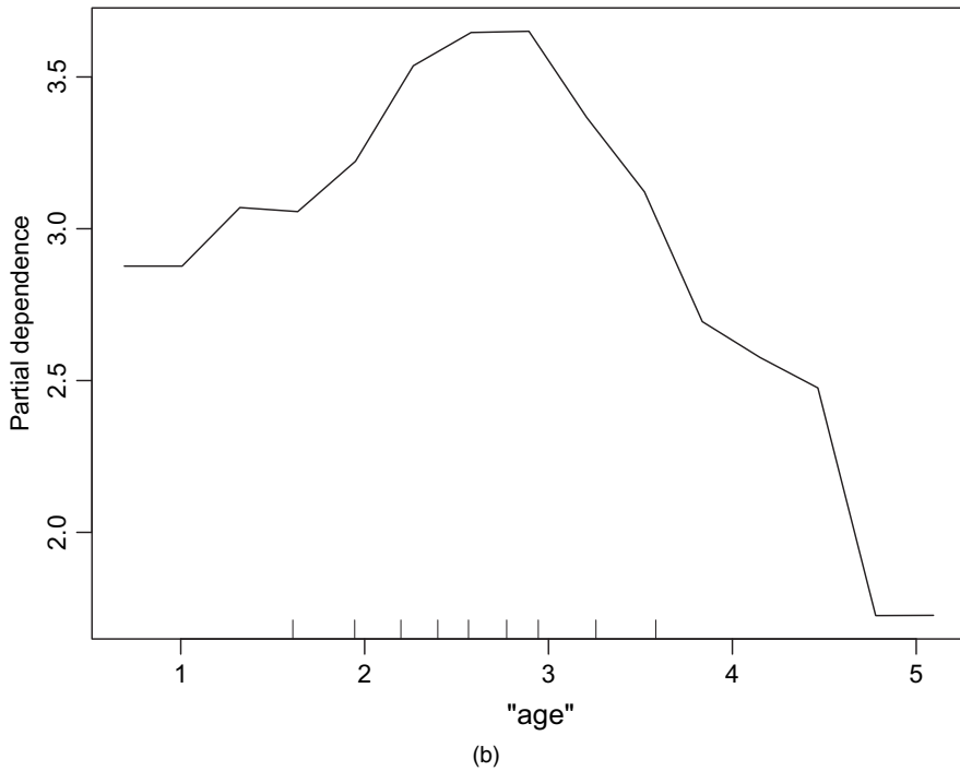
Fig. 6. Random forests for model IV fitted on the full data: (a) variable importance based on Gini impurity; (b) partial dependence plot on age
