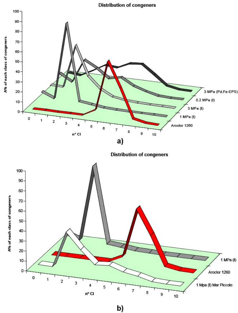
Fig. 1. Hydrodechlorination of Aroclor 1260 results compared with previous best results [5]: a) in pure water; b) diluting Aroclor 1260 in polluted sea water of Mar Piccolo
