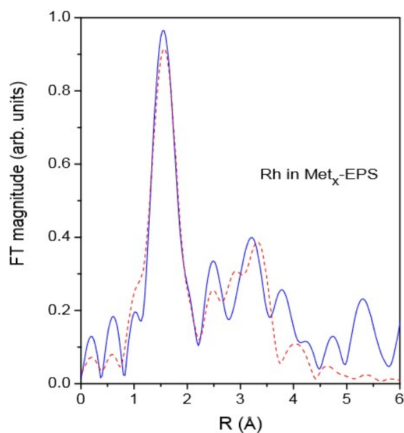
Fig. 6. Fourier transform magnitude of k 2 -weighted Rh K-edge EXAFS spectra of Rh in Met x -EPS sample, calculated in the k range 3–11 Å -1 and R range 1–3.4 Å. Experiment: solid line; best-fit EXAFS model of the nearest coordination shells: dashed line.
