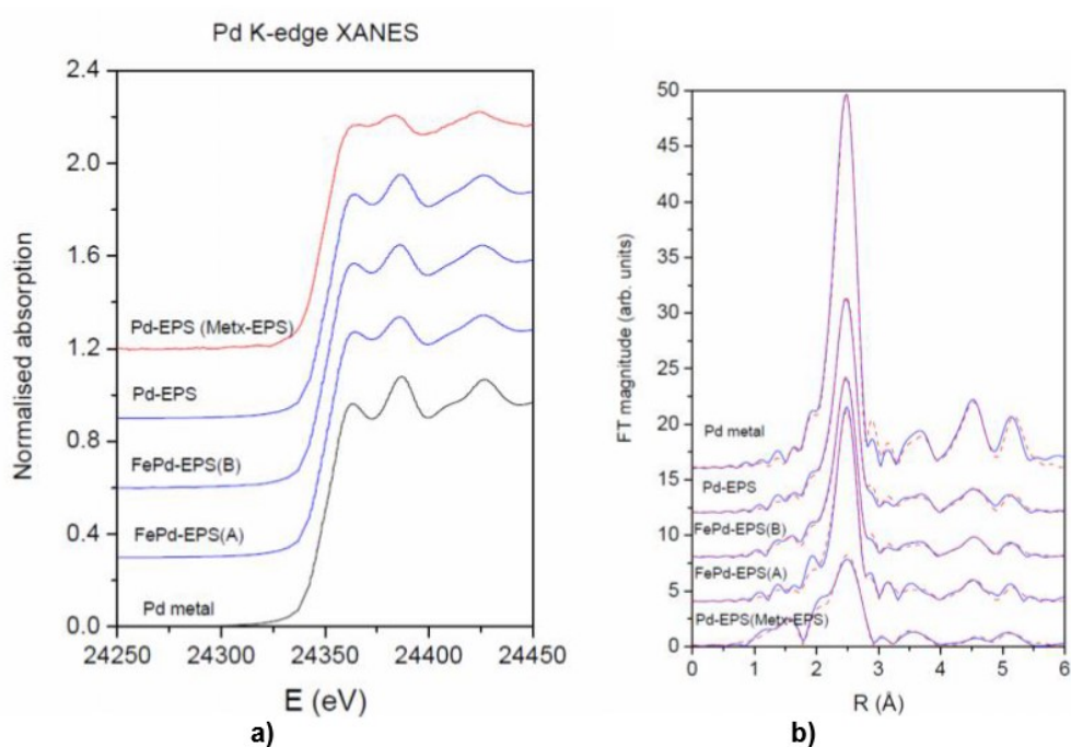
Fig. 2. a) Pd K-edge XANES spectra of the Pd-species in Met x -EPS sample compared to Pd-EPs, FePd-EPs(A), FePd-EPs(B) samples and reference Pd metal foil with f.c.c. crystal structure; b) Pd EXAFS Fourier transform magnitude of k 3 -weighted Pd EXAFS spectra of Pd-EPs, FePd-EPs(A), FePd-EPs(B), Pd-species in Met x -EPS samples and Pd metal foil, calculated in the k range 3–16 Å -1 and R range 1–5.5 Å . Experiment: solid line; best-fit EXAFS model of the nearest coordination shells: dashed line
