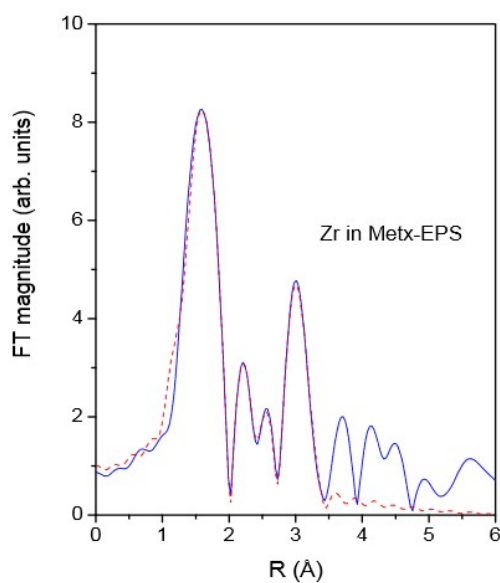
Fig. 5. Fourier transform magnitude of k 3 -weighted Zr K-edge EXAFS spectra of Zr in Met x -EPS sample, calculated in the k range 3–11 Å -1 and R range 1–3.4 Å. Experiment: solid line; best-fit EXAFS model of the nearest coordination shells: dashed line.
