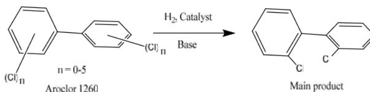
Scheme 1. Hydrodechlorination of Aroclor 1260
