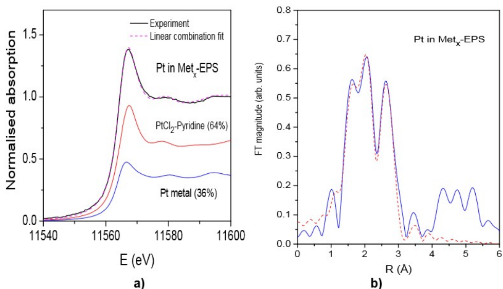
Fig. 3. a) Pt L3-edge XANES spectrum measured on the Pt in Met x -EPS sample: Black solid line: experiment; magenta dashed line: best-fit linear combination of XANES profiles of Pt fcc metal (36%), and cis-dichlorobis pyridine platinum reference compound (64%); b) Fourier transform magnitude of k^2 -weighted Pt L3-edge EXAFS spectra of Pt in Met x -EPS sample, calculated in the k range 3–12 Å -1 and R range 1–3.8 Å. Experiment: solid line; best-fit EXAFS model of the nearest coordination shells: dashed line.
