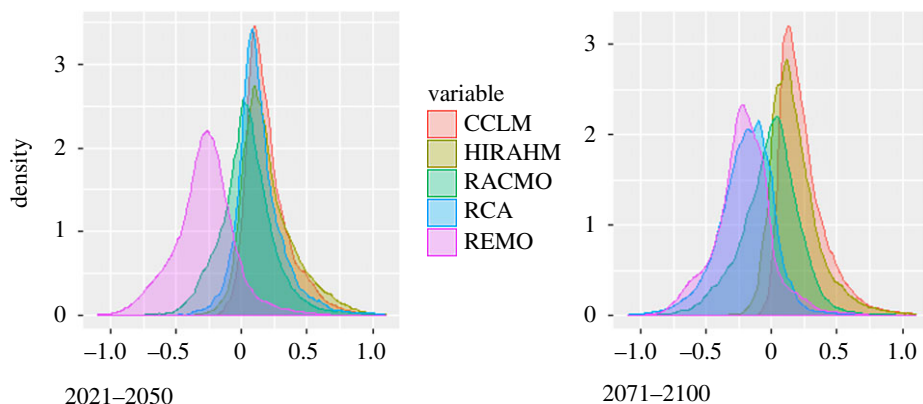
Figure 5. Density distribution of the CPI scores by different RCMs.
