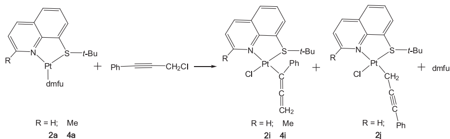
Scheme 4. Oxidative addition of 3-chloro-1-phenylpropyne on complexes 2a and 4a .
