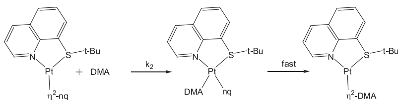
Scheme 6. Proposed mechanism involving an intermediate bearing the leaving olefin and the entering alkyne simultaneously coordinated.
