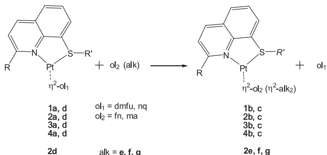
Scheme 5. Olefin-olefin or olefin-alkyne exchange reaction.
