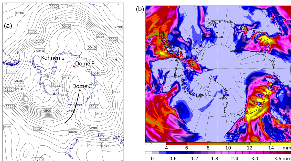
Figure 5. (a) 500 hPa geopotential height from AMPS archive data (Domain 1) 13 September 2009 00:00 GMT. The axis of the upper-level ridge mentioned in the text is marked by a bold black line. (b) 24 h precipitation from AMPS 13 September 2009 00:00 to 24:00 GMT.
