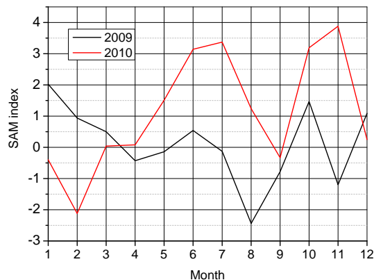
Figure 8. Mean monthly SAM index for 2009 and 2010 (after Marshall, 2003).
