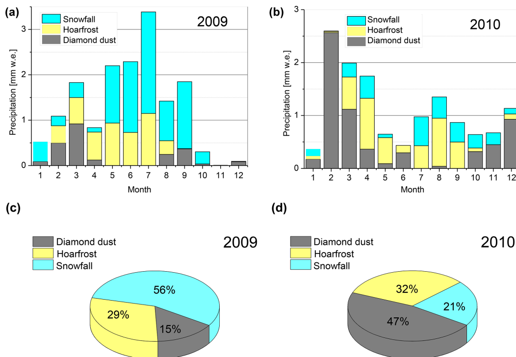
Figure 4. Monthly precipitation at Dome C (a) 2009 and (b) 2010, distinguishing three different types of precipitation: diamond dust, hoarfrost, and snowfall. Relative frequency of diamond dust, hoarfrost, and snowfall for (c) 2009 and (d) 2010. The types were determined from photos of the crystals on the platforms by the Avalanche Research Institute, Arabba, Italy.
