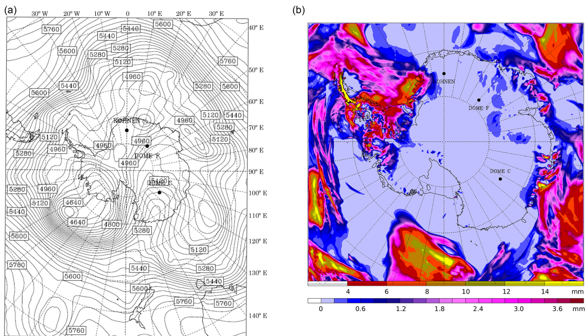
Figure 6. Example for synoptic situation, during which precipitation is observed at Dome C, but not forecast by WRF in AMPS. (a) 500 hPa geopotential height, Domain 2. (b) 24 h precipitation total (mm) from AMPS.
