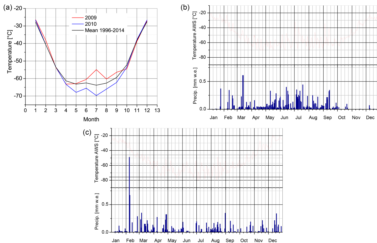
Figure 3. (a) Mean monthly temperatures for 2009 and 2010 at Dome C AWS. (b) Daily precipitation and daily mean temperature at Dome C for 2009 and 2010.
