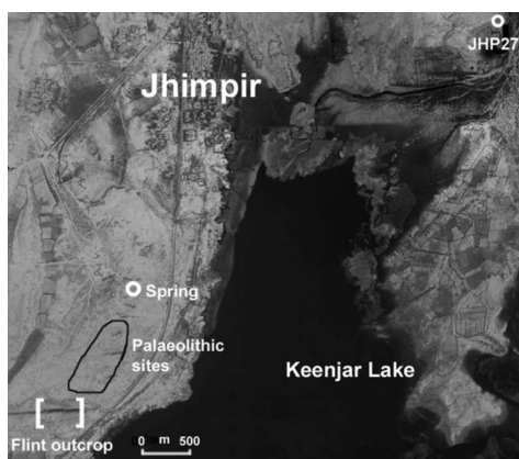
Plate 2 Jhimpir: distribution map of the Final Palaeolithic find spots, on the limestone terraces facing the present-day shore of Keenjar Lake, between a freshwater spring, in the north, and a flint source, in the south. JHP27 locates a microbladelet flint core (map by P. Biagi).
