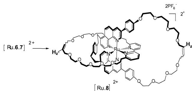
Figure 4. Double RCM leading to the catenane [\text{Ru}(\text{bpy})_2(\text{bpy})]^{2+} .
