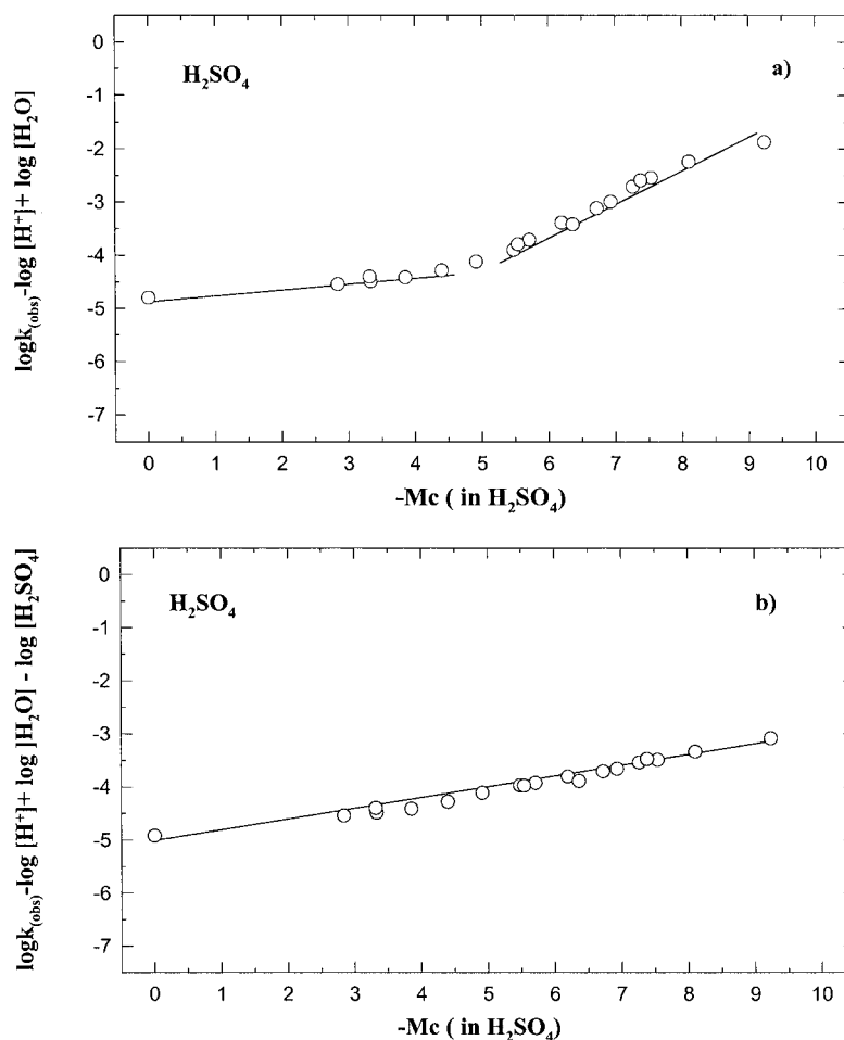
Figure 3 Beckmann rearrangement of 2,4,6-trimethylacetophenone oxime in \text{H}_2\text{SO}_4 (range 52–98 wt%) at 25^\circ\text{C} : a) Plot of \{\log k_{\text{obs}} - \log [\text{H}^+] + \log [\text{H}_2\text{O}]\} vs \text{Mc} . b) Plot of \{\log k_{\text{obs}} - \log [\text{H}^+] + \log [\text{H}_2\text{O}] - \log [\text{H}_2\text{SO}_4]\} vs \text{Mc} ; intercept = -4.8 , slope = 0.18 . Values of \log k_{\text{obs}} for the formation of intermediate from Ref. [7] and present work. Values of \text{Mc} and \log [\text{H}^+] from Ref. [13].
