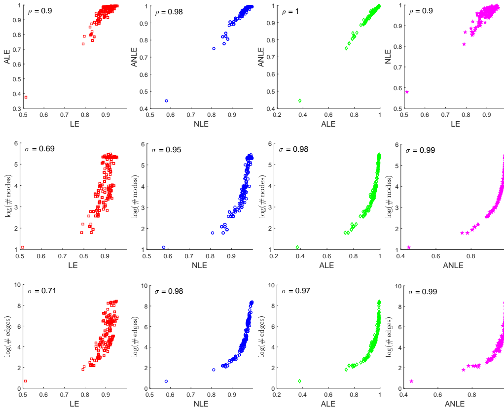
Figure 4.16: Correlation between entropies (top), entropy and number of nodes (middle) and edges (bottom) on the PPI dataset.
