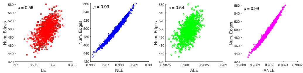
Figure 4.8: Entropies correlations on the Erdős-Rényi graphs for p = 0.1 (top), p = 0.4 (middle), and p = 0.7 (bottom).
