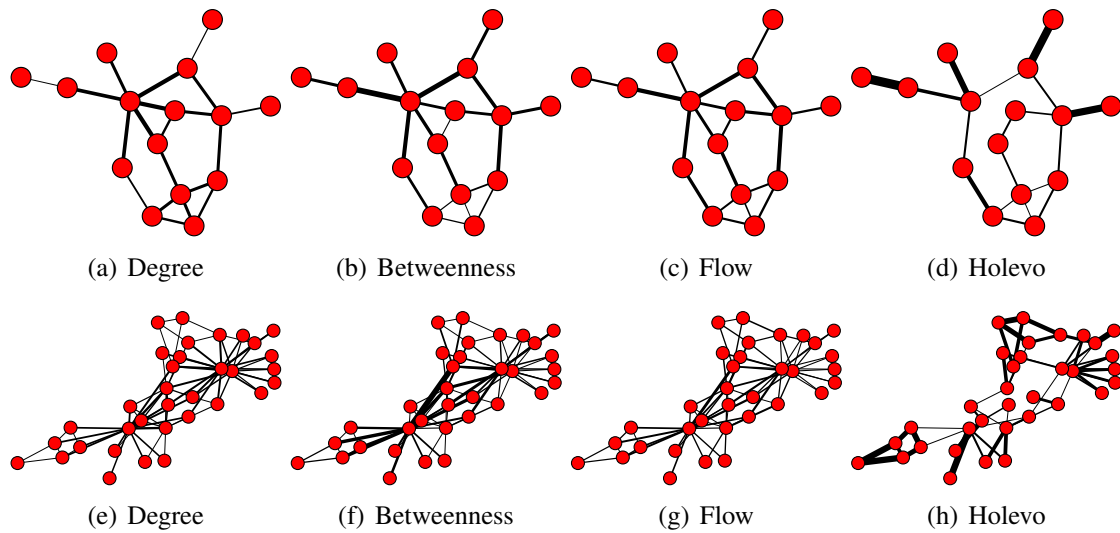
Figure 4.18: Edge centralities on the Florentine families network (a-d) and the Karate club network (e-h). A thicker edge indicates a higher value of the centrality.
