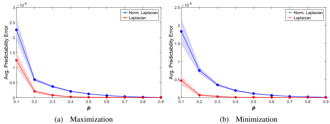
Figure 4.12: Average predictability error ( \pm standard error) on Erdős-Rényi graphs.
