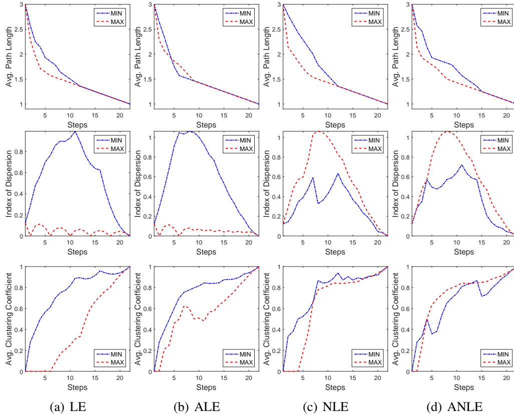
Figure 4.4: Top-to-bottom: Average path length, index of dispersion, and average clustering coefficient at different steps of the temporal evolution of the graphs in Fig. 4.1.
