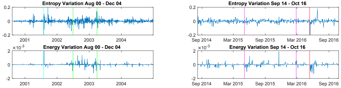
Figure 5.1: USSM dataset - Entropy and Energy variation vs time, respectively top and bottom chart. The vertical coloured lines mark some important events for the trade market: September 11 attacks, Downturn of 2002-2003, Financial Crisis of 2007-2008, Dow Jones lowest point (March 2009), Stock Markets Fall (August 2011), Greek legislative election (June 2012), United States debt-ceiling crisis (October 2013), Chinese stock market turbulence 2015, Brexit Referendum (June 2016).
