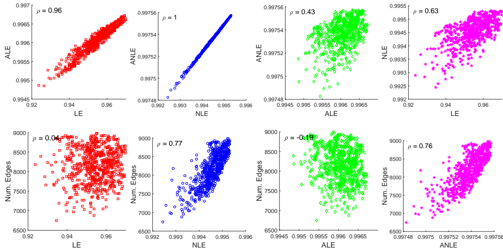
Figure 4.15: Correlation between the entropies (top) and entropy and number of edges (bottom) on the USSM dataset.
