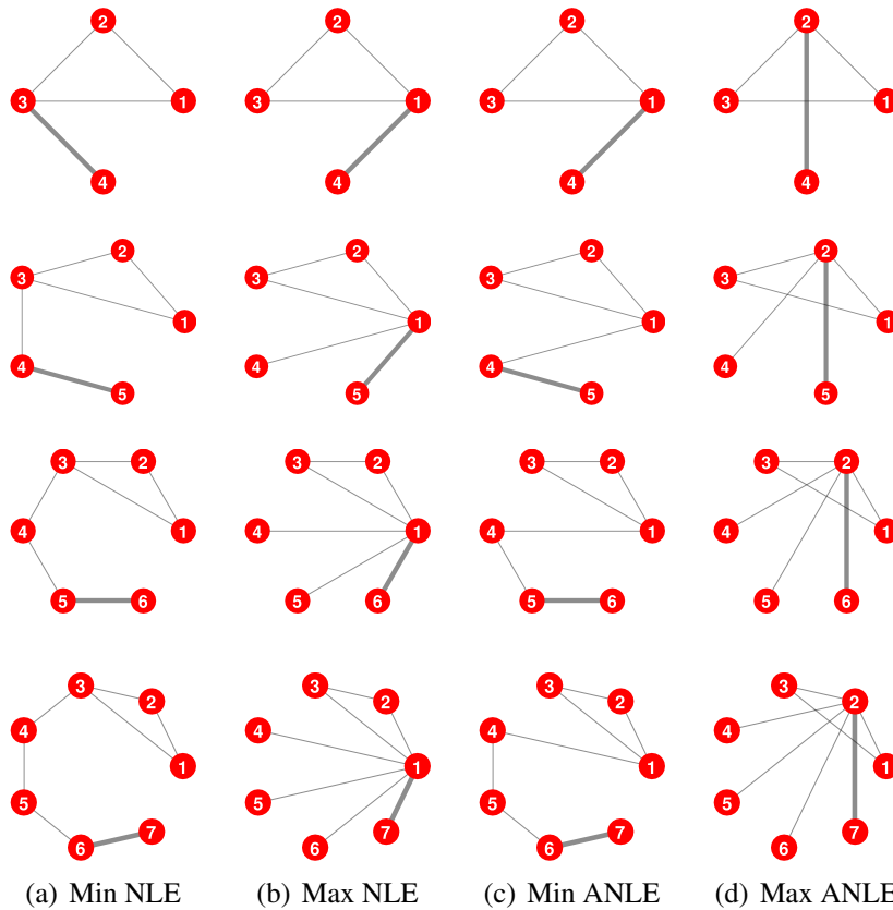
Figure 4.6: Evolution of the graph structure when we iteratively add a new node and we connect it to the graph so as to (a) minimize and (b) maximize the normalized Laplacian entropy (NLE). (c) and (d) show similar results for the approximate normalized Laplacian entropy (ANLE). Here the seed graph is a clique over 3 nodes.
