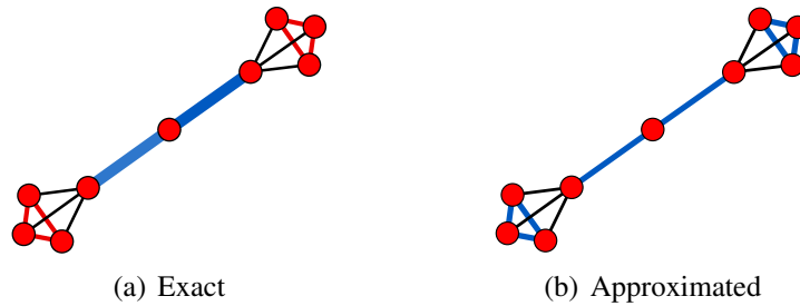
Figure 4.17: The Holevo edge centrality and its quadratic approximation on a barbell graph. Here the edge thickness is proportional to the value of the centrality. In (a) the blue edges have a higher centrality than the red edges, but in (b) all these edges (blue) have the same degree centrality.
