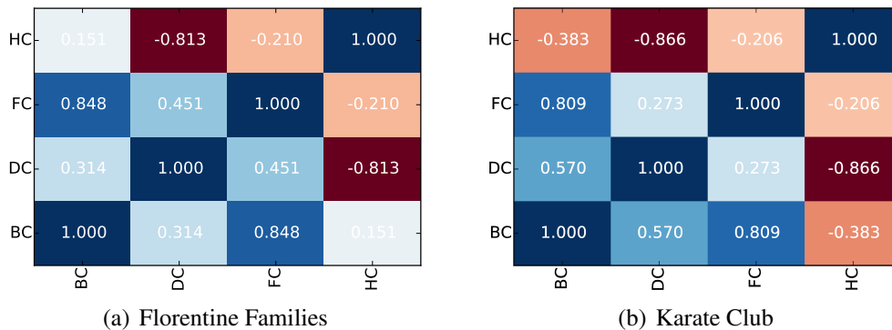
Figure 4.19: Correlation matrices for the centrality measure on the Florentine family network and the karate club network. DC, BC, FC, and HC denote the degree, betweenness, flow and Holevo centralities, respectively.
