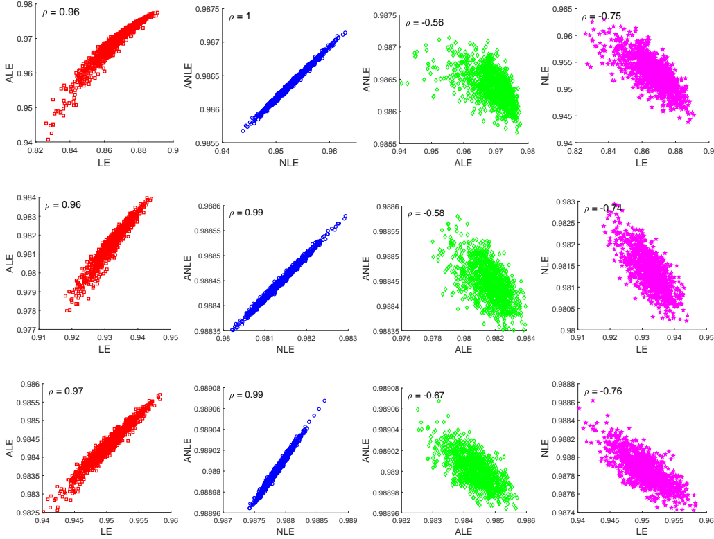
Figure 4.10: Entropies correlation on the scale-free graphs for m = 1 (top), m = 3 (middle), and m = 5 (bottom).
