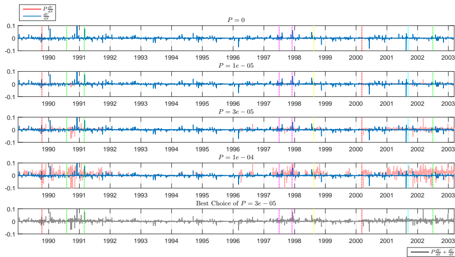
Figure 5.7: NYSE dataset - Temperature components vs time, as pressure changes. The vertical coloured lines indicate important events for the trade market: Friday the 13th Mini-Crash (October 1989), Persian Gulf War (August 1990 – January 1991), Asian Financial Crisis (July 1997 – October 1997), Russian Financial Crisis – Ruble devaluation (August 1998), Dot-com bubble - climax (March 2000), September 11 attacks, Downturn of 2002-2003.
