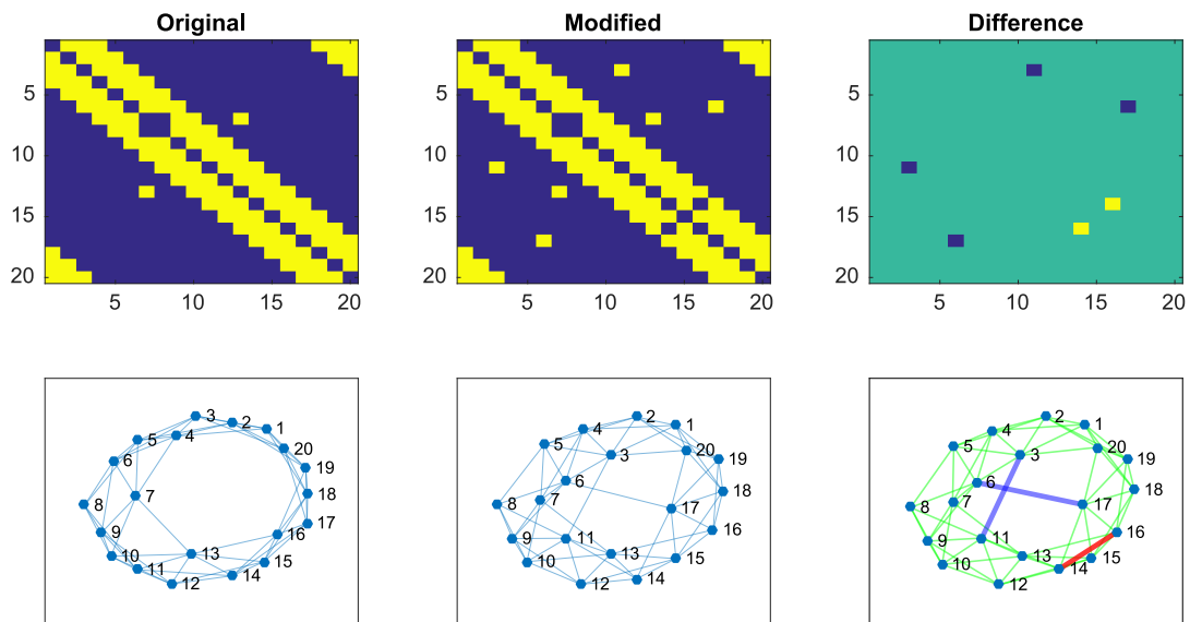
Figure 4.21: Perturbation process: on the left, adjacency matrix and plot of the starting graph; in the middle, the edited graph; on the right, the differences between initial and modified graph are highlighted.
