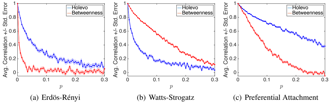
Figure 4.22: Average correlation between the centrality of the edges of the original graph and those of increasingly noisy version of it. The different columns refer to different starting graphs: (a) Erdős-Rényi, (b) Watts-Strogatz and (c) Preferential Attachment.
