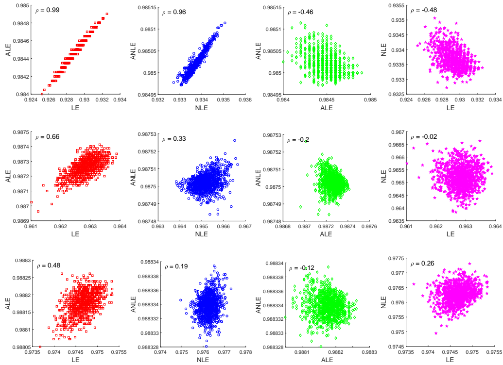
Figure 4.11: Entropies correlation on the small-world graphs for k = 2 (top), k = 4 (middle), and k = 6 (bottom).
