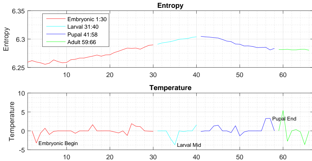
Figure 5.6: Drosophila Melanogaster dataset - Entropy and Temperature vs time, respectively top and bottom. The developmental periods of the fruit fly are coloured differently and the significant moments are highlighted.
