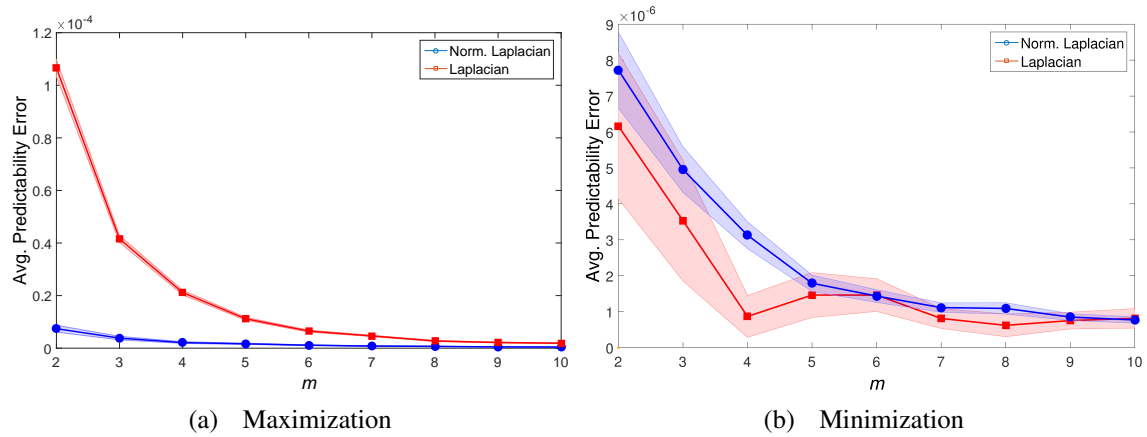
Figure 4.13: Average predictability error ( \pm standard error) on scale-free graphs.
