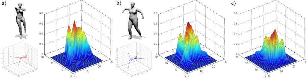
Figure 3.2: An example of the effect of Orthogonal transformation over the eigenvector matrix. In the left-hand side panel a) the reference mesh - the graph below the mesh shows the plot of the first three non trivial eigenvectors of the reference mesh whereas on the right of the mesh there is the kernel density estimation computed on the eigenvector matrix. In the middle panel b) the mesh to be aligned according to a) . Finally, in the right-hand side panel c) the result of the optimization process.
