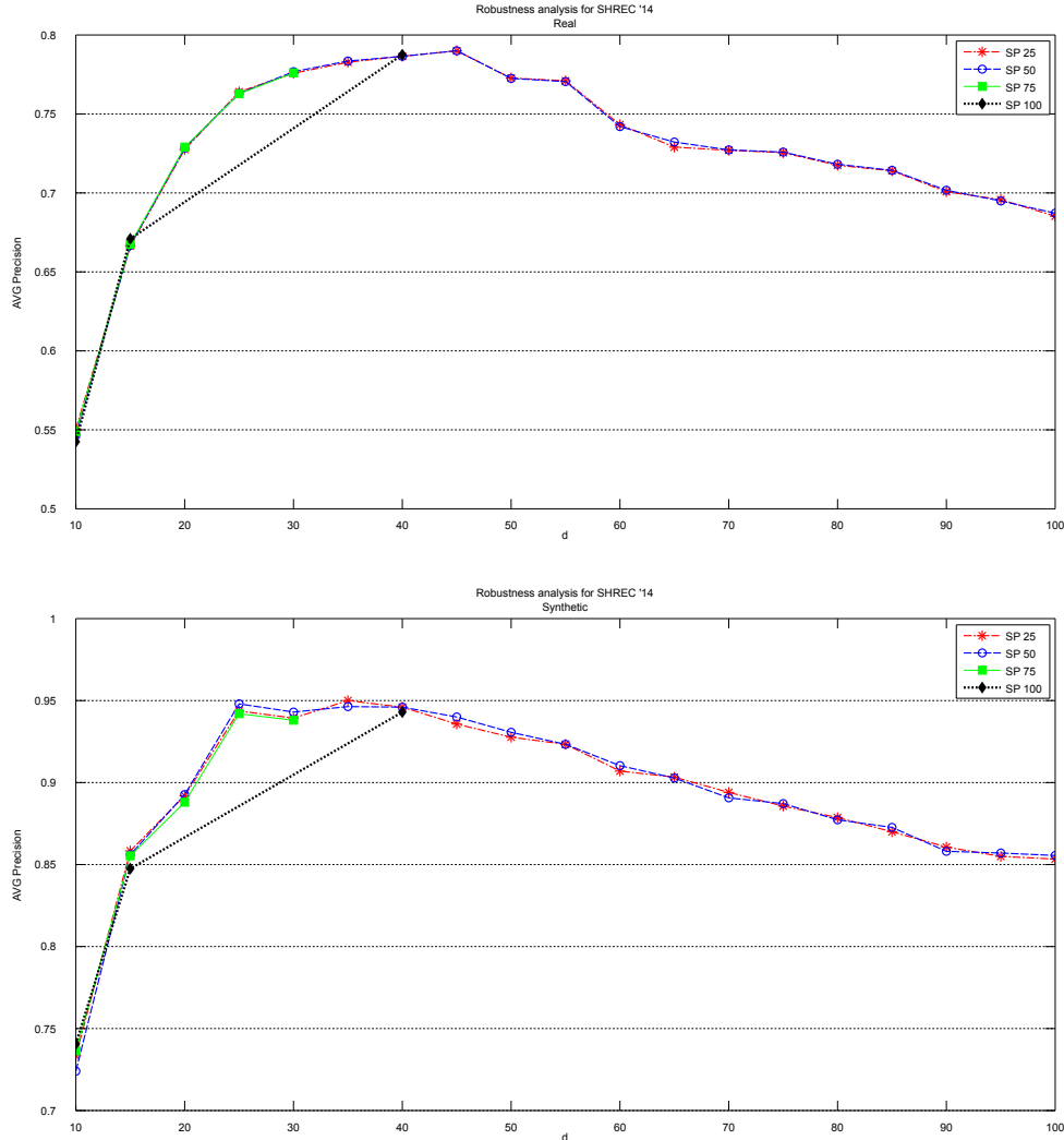
Figure 3.4: Robustness analysis of the proposed method in both Real (top) and Synthetic (bottom) datasets. The marks represent the average precision obtained with a certain embedding dimension. Different lines represent different sub-sampling percentage, e.g. , the red line represents the average accuracy with respect to different embedding dimensions after removing 75% of the data on the model ( i.e. , keeping only 25% of the data).
