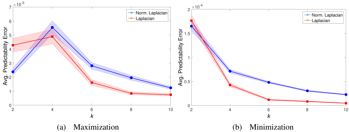
Figure 4.14: Average predictability error ( \pm standard error) on small-world graphs.
