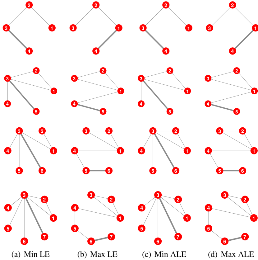
Figure 4.5: Evolution of the graph structure when we iteratively add a new node and we connect it to the graph so as to (a) minimize and (b) maximize the Laplacian entropy (LE). (c) and (d) show similar results for the approximate Laplacian entropy (ALE). Here the seed graph is a clique over 3 nodes.
