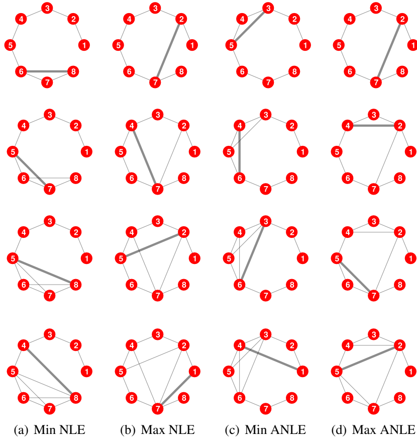
Figure 4.2: Evolution of the edge structure of a path graph over 8 nodes when we iteratively add edges that (a) minimize and (b) maximize the normalized Laplacian entropy (NLE). (c) and (d) show similar results for the approximate normalized Laplacian entropy (ANLE).
