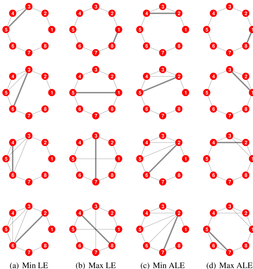
Figure 4.1: Evolution of the edge structure of a path graph over 8 nodes when we iteratively add edges that (a) minimize and (b) maximize the Laplacian entropy (LE). (c) and (d) show similar results for the approximate Laplacian entropy (ALE).
