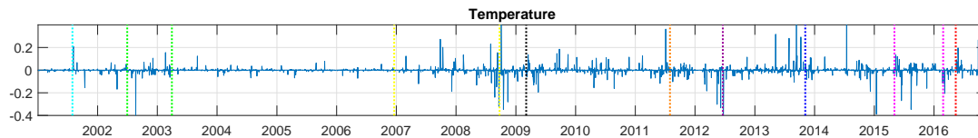
Figure 5.3: USSM dataset - Temperature vs time. The vertical coloured lines refer to some important events for the trade market: September 11 attacks, Downturn of 2002-2003, Financial Crisis of 2007-2008, Dow Jones lowest point March 2009, August 2011 stock markets fall, Greek legislative election June 2012, United States debt-ceiling crisis October 2013, Chinese stock market turbulence 2015-16, Brexit Referendum June 2016.
