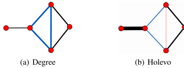
Figure 4.20: Toy example showing the difference in the structural information captured by the degree and Holevo centralities.
