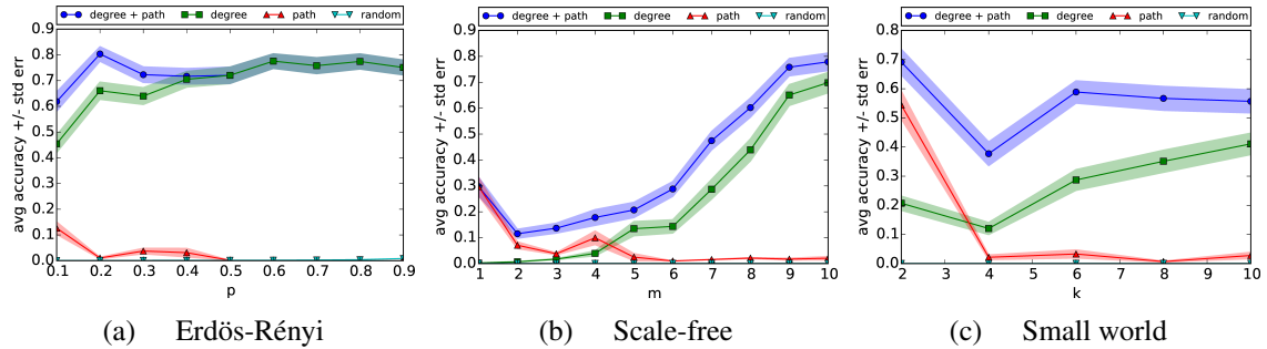
Figure 4.3: Average accuracy when predicting the edge whose addition maximizes the Laplacian entropy when using four different heuristics, i.e., choose (1) the pair of nodes with minimum degree sum; (2) the pair of nodes with maximum geodesic distance; (3) the pair of nodes with minimum degree sum and maximum geodesic distance; (4) a pair of nodes u and v picked at random, with (u, v) \notin E .
