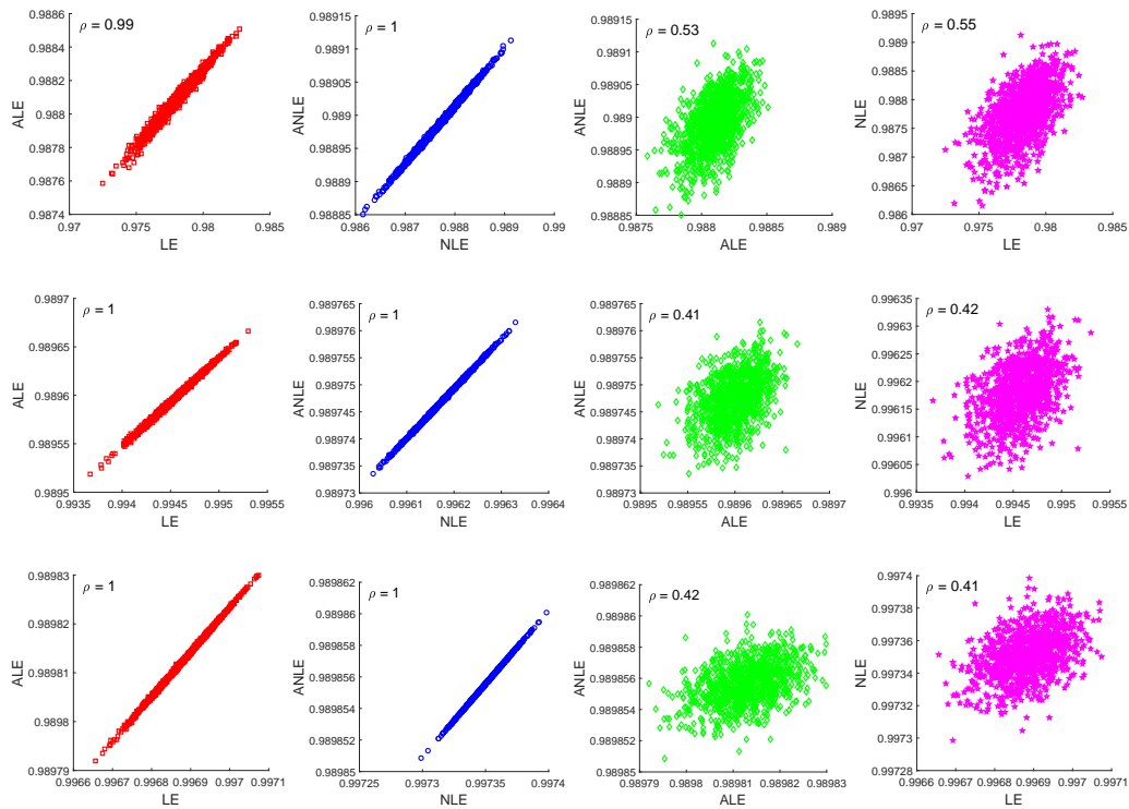
Figure 4.8: Entropies correlations on the Erdős-Rényi graphs for p = 0.1 (top), p = 0.4 (middle), and p = 0.7 (bottom).
