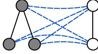
Figure 4.23: Given two graphs G_1(V_1, E_1) and G_2(V_2, E_2) we construct a new graph \mathcal{G} = (\mathcal{V}, \mathcal{E}) where \mathcal{V} = V_1 \cup V_2 , \mathcal{E} = E_1 \cup E_2 and we add a new edge (u, v) between each pair of nodes u \in V_1 and v \in V_2 .
