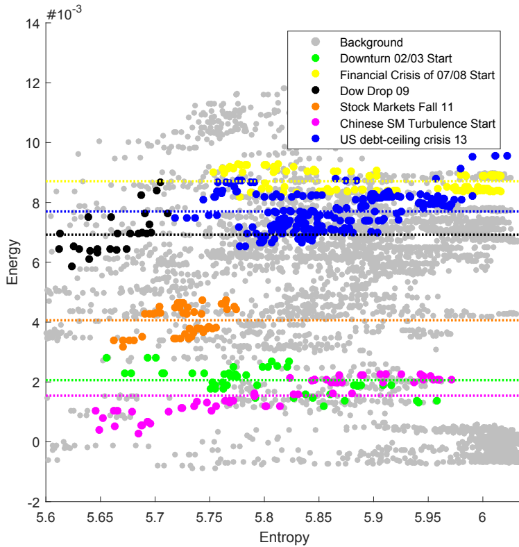
Figure 5.5: USSM dataset - Scatter plot of Energy ( U ) over Entropy ( S ). Each dot is a day and grey dots are the background. Dots of the same color belong to the same network phase. Horizontal lines represent cluster centroids for the energy dimension.
