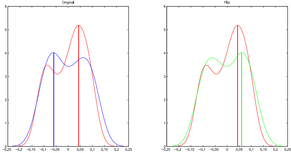
Figure 3.1: The red curve is the pdf of the i -th eigenvector of matrix A (reference mesh), calculated with the kernel density estimation, and the blue curve is the pdf of the i -th eigenvector of matrix B. On the right, the green curve represents the pdf after the sign flip.
