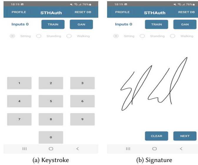
Figure 2: Data Collection Interface
