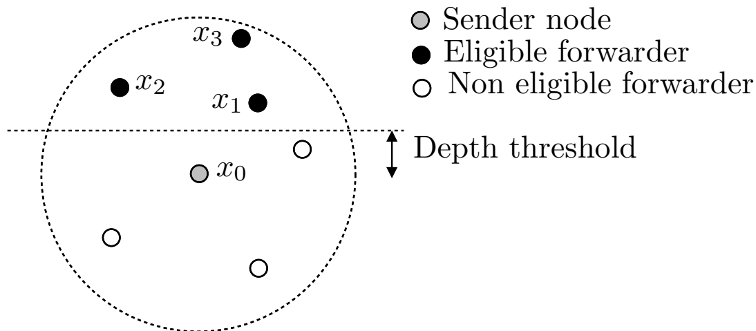
Figure 7.1.: Sketch of a transmission in DBR.
