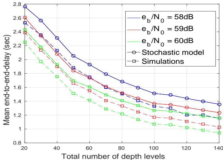
Figure 5.15.: Comparison of stochastic model and Monte-Carlo simulation for Mean end-to-end delay (sec)
