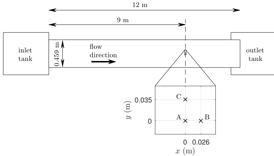
Figure 1 Schematic of the experimental flume. The inset shows the spatial arrangement of the three conductance wave probes.
