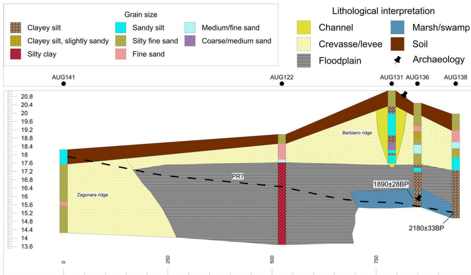
Figure 11. W-E cross section (CS2) in correspondence with the Barbiano ridge (the dashed line indicates uncertainty in the stratigraphic correlation).
