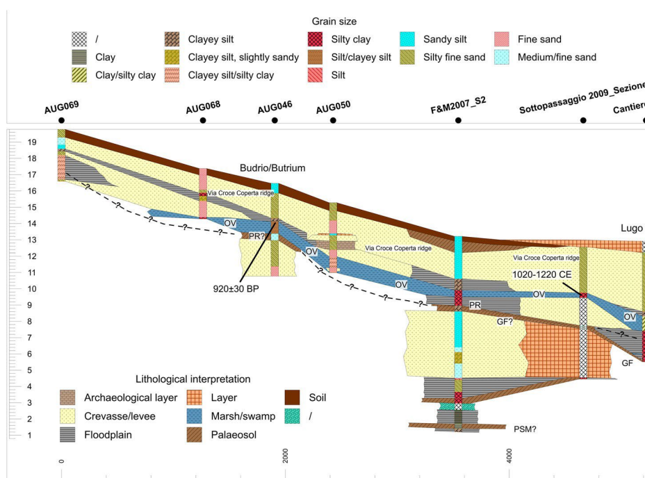
Figure 13. Eastern S-N cross section (CS4) between Budrio and Lugo (PR = Roman palaeosol; GF = Geosuolo Formellino; OV = Orizzonte Veggiani; PSM = stands for Palaeosuolo San Martino, a palaeosol associated with the Neolithic occupation of the area; the dashed lines indicate uncertainty in the stratigraphic correlations).
