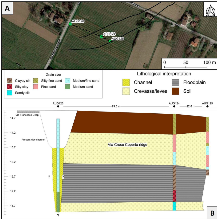
Figure 9. Detailed view of fluvial traces pertaining to Via Croce Coperta palaeochannel with augers location (A) and stratigraphic cross section (B) up to Via F. Crispi (Google Satellite basemap, Copyright © Google).
