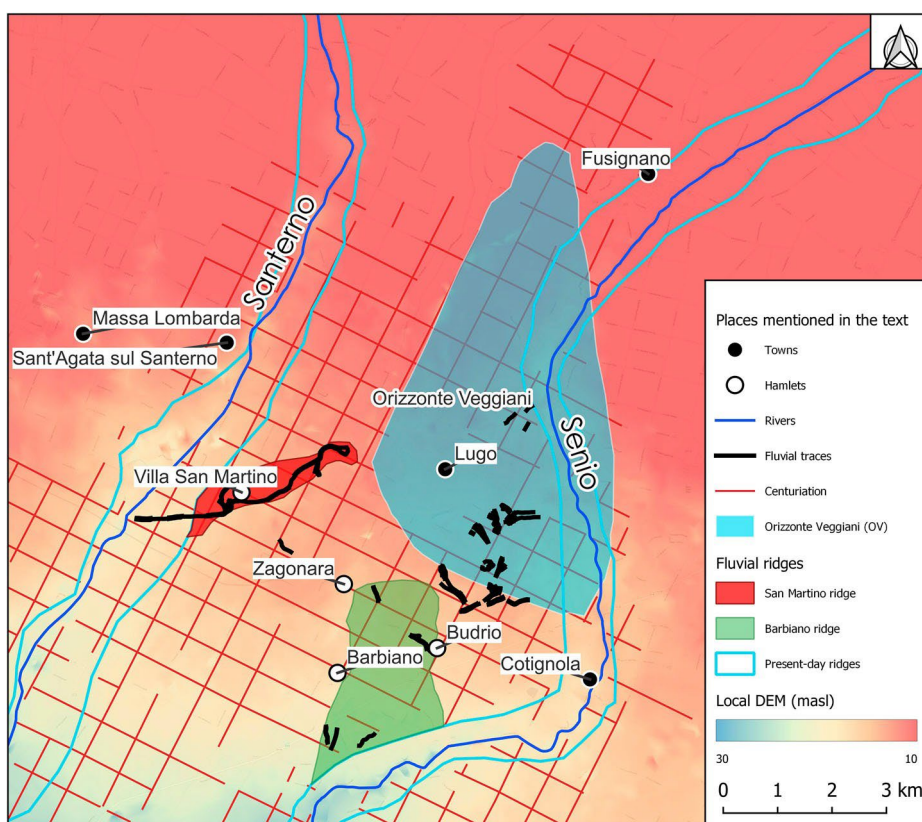
Figure 2. Study area with main rivers, remains of the ‘centuriation’, main geomorphological elements, including the extension of the Orizzonte Veggiani as reconstructed by Franceschelli and Marabini 2007 and main ridges reassessed through morphometric algorithms according to Abballe and Cavalazzi 2021, and fluvial traces mapped by remote sensing (sources used are listed in Table 2). Local DEM shown as basemap was produced by the author interpolating manually recorded elevation points (for methodology see Abballe and Cavalazzi 2021).
