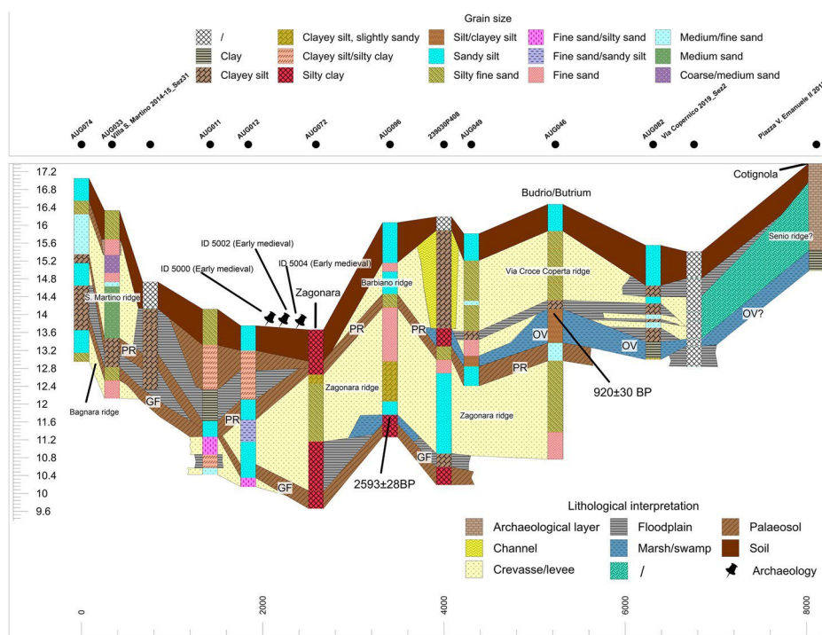
Figure 10. W-E stratigraphic cross section (CS1) across the plain between Santerno and Senio rivers (PR = Roman palaeosol; GF = Geosuolo Formellino; OV = Orizzonte Veggiani).
