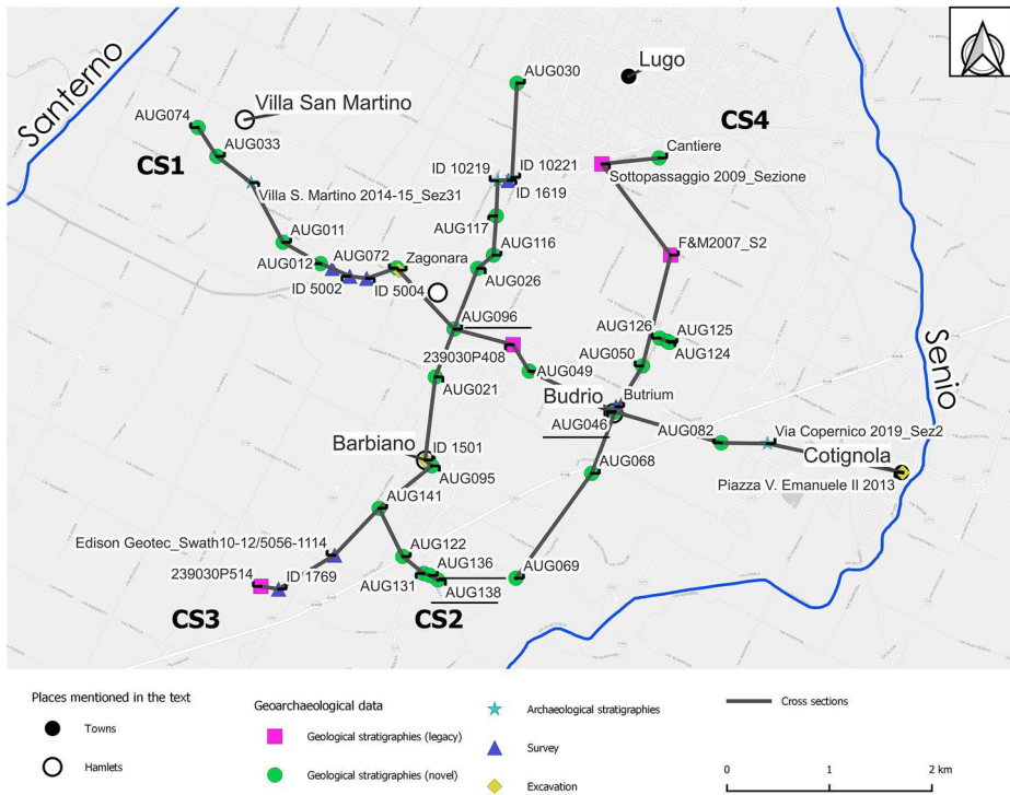
Figure 8. Geoenvironmental investigations with four main stratigraphic transects (CS1-CS4) and archaeological sites considered. Underlined augering names indicate provenance of radiocarbon dated samples (Esri basemap, Copyright © Esri).
