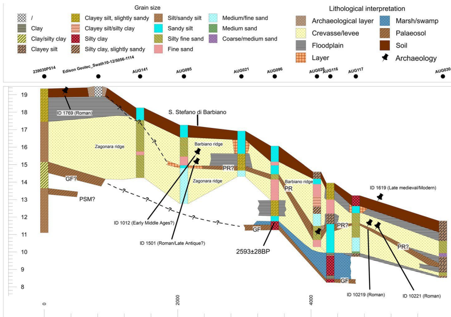
Figure 12. Western S-N cross section (CS3) between Barbiano and Lugo (PR = Roman palaeosol; GF = Geosuolo Formellino; OV = Orizzonte Veggiani; PSM = Palaeosuolo San Martino , a palaeosol associated with the Neolithic occupation of the area; the dashed line indicates uncertainty in the stratigraphic correlation).
