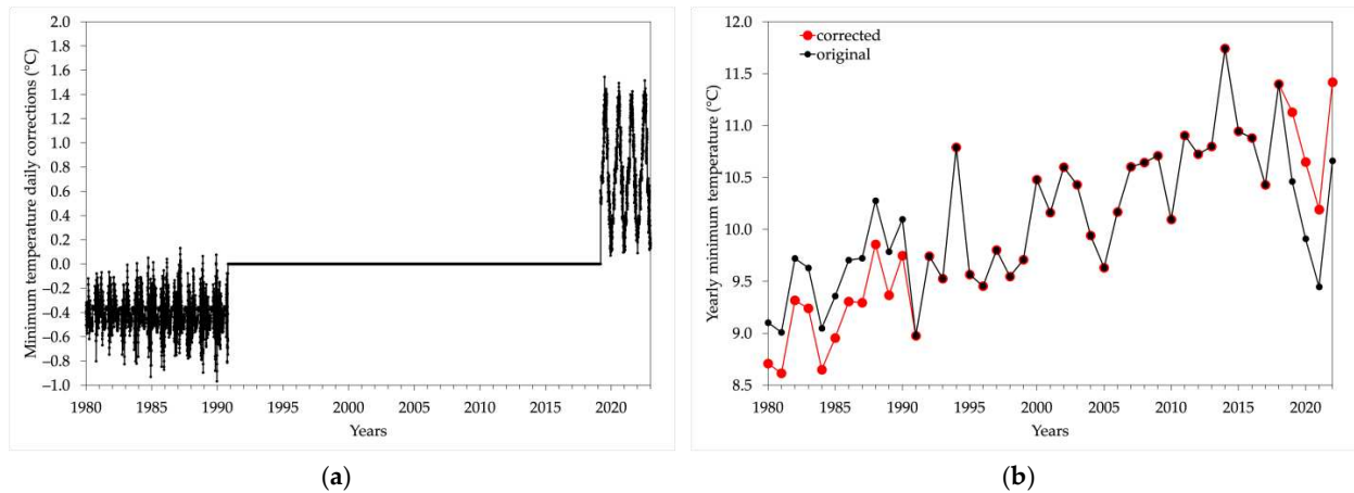
Figure 2. (a) Daily corrections applied to minimum temperature. (b) Yearly mean of the original series (black) and the corrected one (red).
