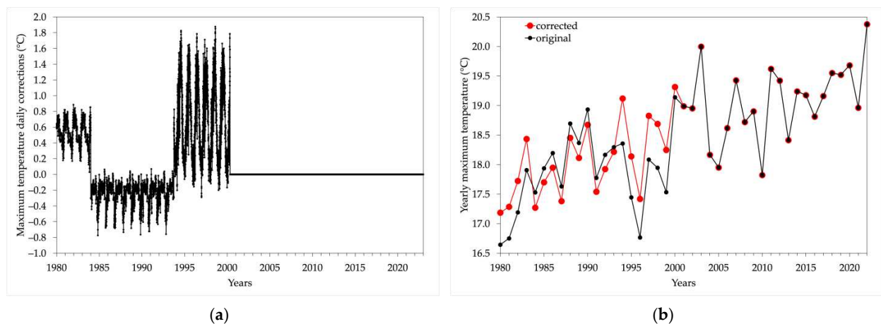
Figure 3. (a) Daily corrections applied to maximum temperature. (b) Yearly mean of the original series (black) and the correction (red).
