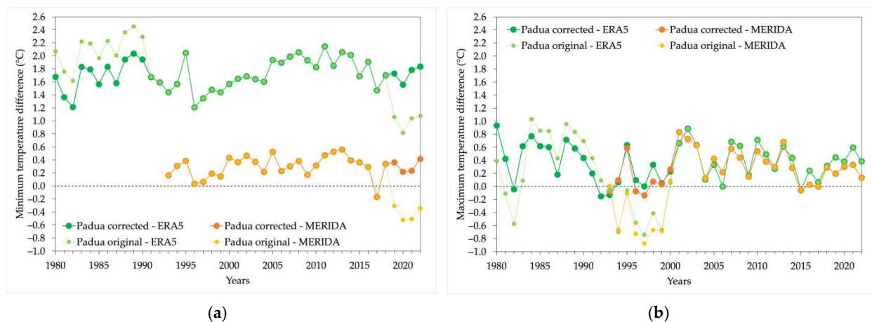
Figure 4. (a) Difference of yearly minimum temperatures between the Padua, original and corrected, and ERA5 series over 1980–2022 (green) and between MERIDA over 1993–2022 (orange). (b) The same but for maximum temperature. The continuous lines highlight the zero value.
