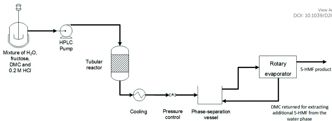
Figure 4. Biphasic continuous process for 5-HMF production from fructose: biphasic system of water/DMC with HCl as catalyst and fructose were pre-mixed and pumped into a tube reactor under pressure at T = 180\text{--}200\text{ }^{\circ}\text{C} . Also, the strategy for 5-HMF recovery and purification from both organic and aqueous phase is shown. Reproduced with permission from ref. 103. Copyright 2020 Royal Society of Chemistry.
