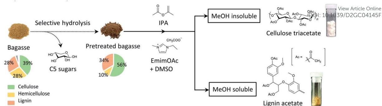
Figure 8. The organocatalytic transesterification of bagasse and the subsequent fractionation into cellulose triacetate and lignin acetate. Reprinted from "A mechanistic insight into the organocatalytic properties of imidazolium-based ionic liquids and a positive co-solvent effect on cellulose modification reactions in an ionic liquid" R. Kakuchi, R. Ito, S. Nomura, H. Abroshan, K. Ninomiya, T. Ikai, K. Maeda, H. J. Kim and K. Takahashi, RSC Adv. , 2017, 7, 9423-9430 (ref. 175), https://pubs.rsc.org/en/content/articlelanding/2017/ra/c6ra28659c .
