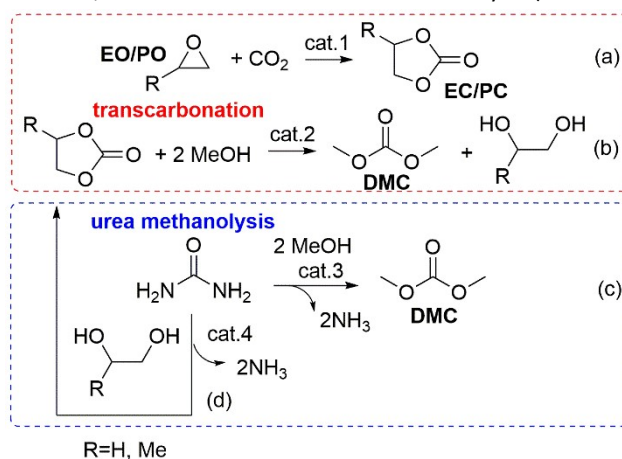
Scheme 1. Synthesis of DMC. Top: CO 2 insertion into epoxides (a) followed by transcarboxylation of alkylene carbonate (b) (red box); bottom: direct and indirect urea methanolysis (c) and (d), respectively (blue box). Cat. 1: bifunctional catalyst, cat. 2: amphoteric catalyst; cat. 3 and 4: amphoteric heterogeneous catalyst.
