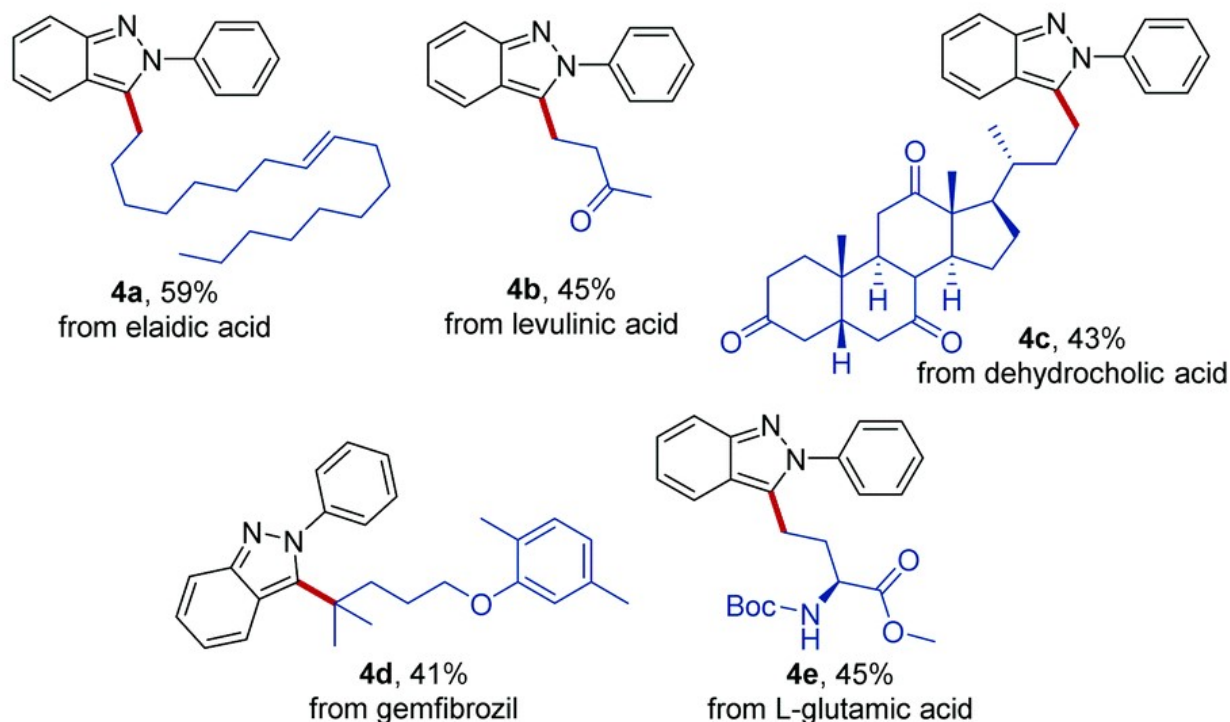
Scheme 11. Late-stage modification of natural resources and drug molecules. Reaction conditions: 1a (0.2 mmol), 2 (2 equiv.), 4CzIPN (5 mol%), DABCO (1 equiv.), DMC (2 mL), T = 35 °C, blue LED, t = 12 h under N 2 atmosphere. Reproduced with permission from ref. 108. Copyright 2021 Chinese Chemical Society (CCS), Shanghai Institute of Organic Chemistry (SIOC), and the Royal Society of Chemistry.
