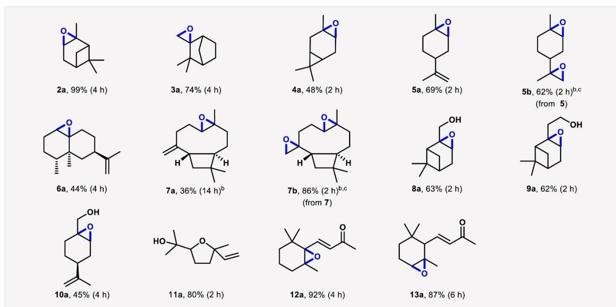
Scheme 10. Cobalt catalysed epoxidation of bio-renewable alkenes (GC yields and reaction times). Substrate (0.5 mmol), isobutyraldehyde (IBA, 1.25 mmol), catalyst (8 mol%, 47 mg), DMC (5 mL), O 2 (1 atm), rt. Conversions were nearly complete in all reactions except those performed to obtain products 3a (78 %), 6a (79 %) and 7a (55 %). b T = 40 °C. c5 equiv. of IBA. Reproduced with permission from ref. 100. Copyright 2022 Elsevier Ltd.
