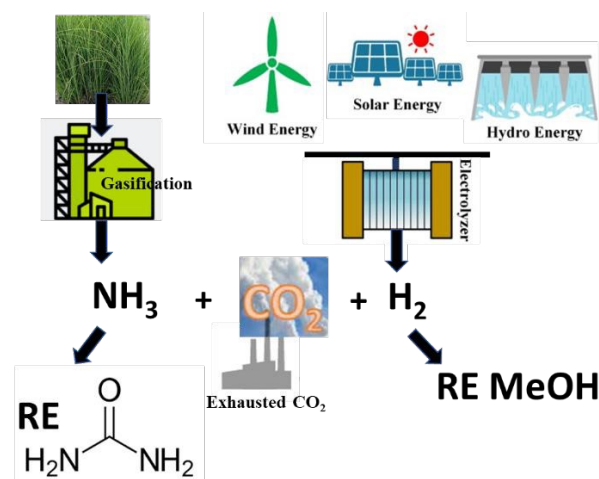
Scheme 2. Sustainable production of MeOH (right) and urea (left) for the synthesis of DMC.
