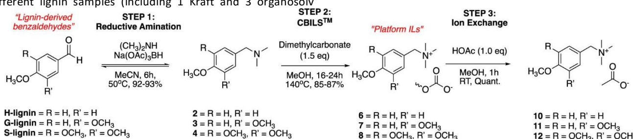
Scheme 20. Three-step synthesis of lignin derived ILS from methylated lignin-derived benzaldehydes. Reproduced with permission from V. Diez, A. DeWeese, R. S. Kalb, D. N. Blauch and A. M. Socha, Ind. Eng. Chem. Res. , 2019, 58 , 16009-16017 (ref. 159). Copyright 2020 American Chemical Society.
