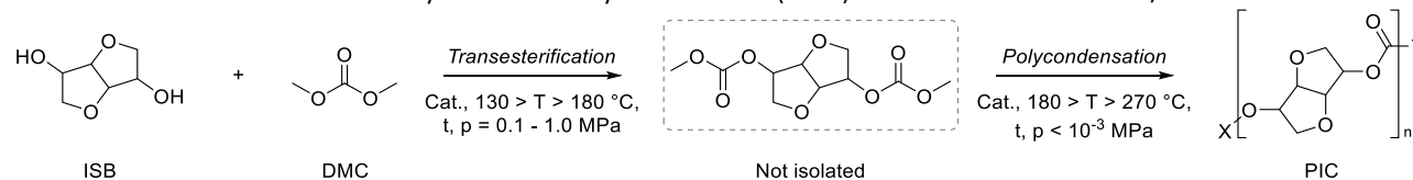
Scheme 17. PIC synthesis via polycondensation of ISB and DMC.
