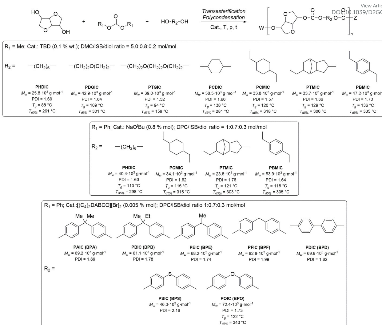
Scheme 18. Diol co-monomers employed for the preparation of isosorbide-based co(polycarbonates).
