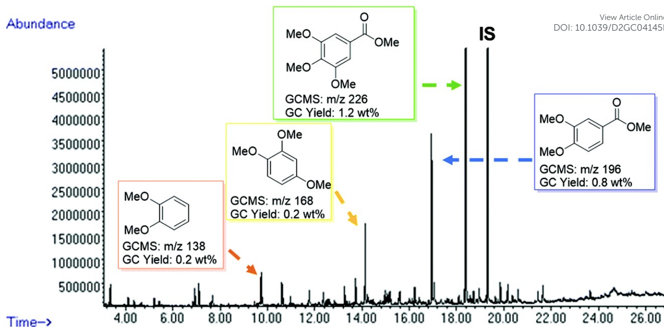
Figure 6. GC-FID trace of the product mixture obtained from the depolymerisation of milled beechwood chips (100 mg) using \text{Cs}_2\text{CO}_3 (10% w/w) in DMC ( V = 5 mL) at T = 180 °C for t = 8 h. Identification of the major peaks is based on the GC-MS data. Quantification is based on the standardization of individual products, using n -octadecane as an internal standard. Reproduced with permission from ref. 162. Copyright 2018 Royal Society of Chemistry.
