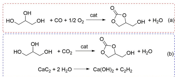
Scheme 8. Synthesis of GC via: (a) catalytic oxidative carbonylation of glycerol (top, red box); (b) direct catalytic insertion of \text{CO}_2 into glycerol in the presence of \text{CaC}_2 as a dehydrating agent (bottom, blue box).
