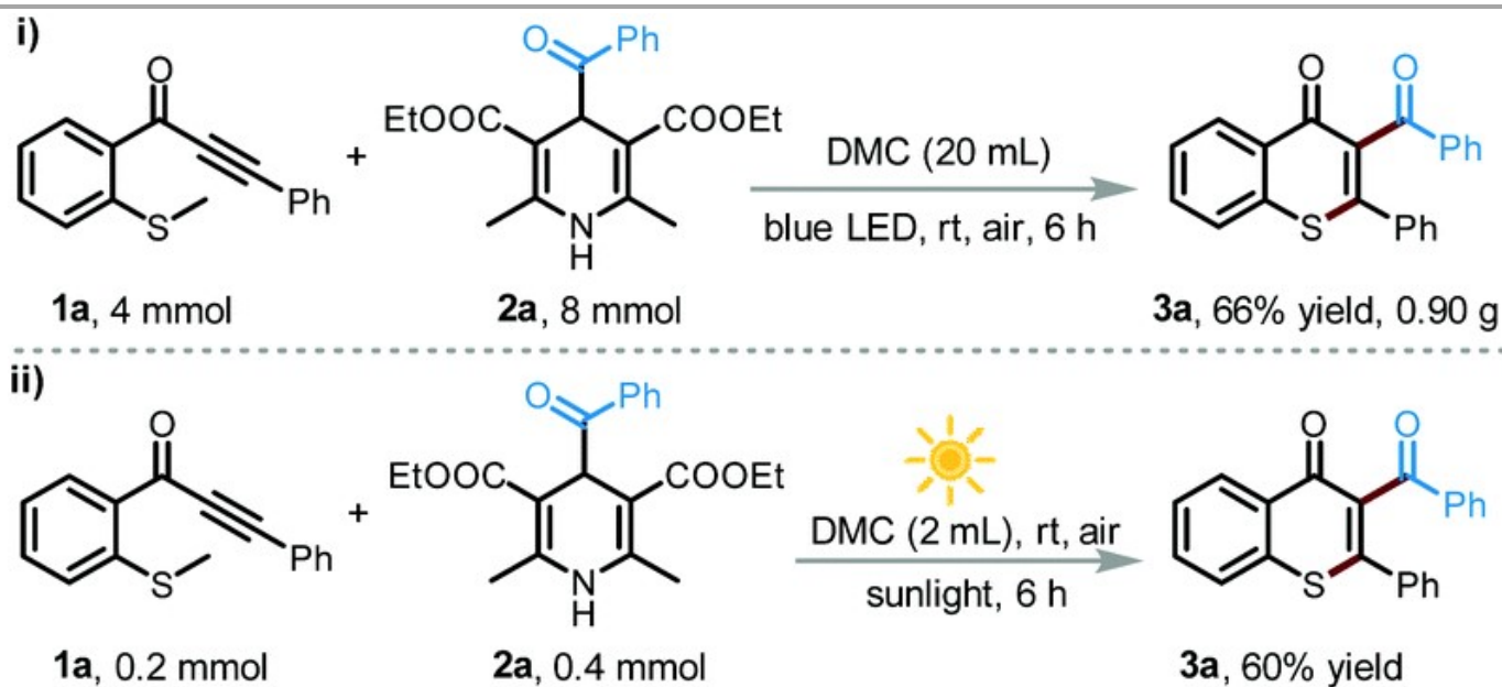
Scheme 11. Late-stage modification of natural resources and drug molecules. Reaction conditions: 1a (0.2 mmol), 2 (2 equiv.), 4CzIPN (5 mol%), DABCO (1 equiv.), DMC (2 mL), T = 35 °C, blue LED, t = 12 h under N 2 atmosphere. Reproduced with permission from ref. 108. Copyright 2021 Chinese Chemical Society (CCS), Shanghai Institute of Organic Chemistry (SIOC), and the Royal Society of Chemistry.
