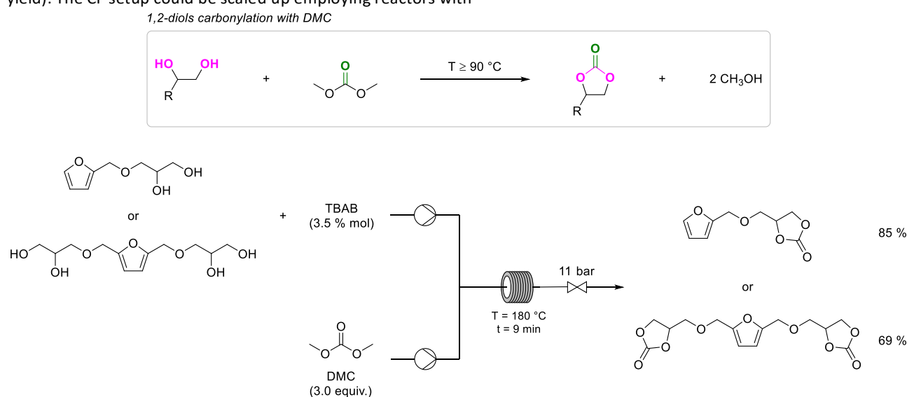
Scheme 15. 1,2-diols carbonylation with DMC (top) and CF carbonylation of FUR and HMF derived 1,2-diols with DMC (bottom). 3.5 mol % of TBAB and 3 equiv. of DMC were added per 1,2-diol functional group. TBAB = tetrabutylammonium bromide. Reproduced with permission from ref. 128. Copyright 2021 Elsevier Ltd.
