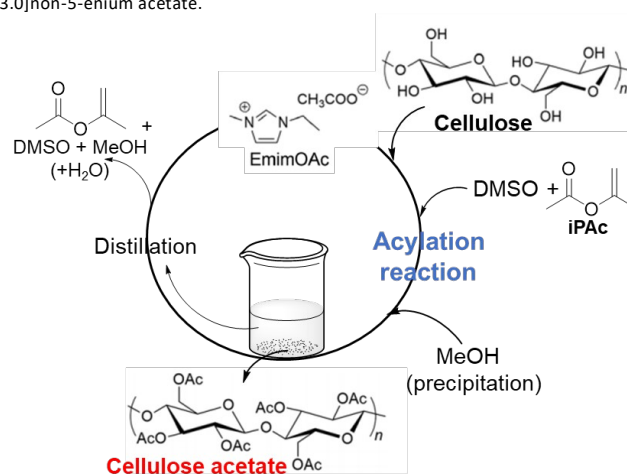
Figure 7. Recycle of the [C 2 C 1 im][OAc]/DMSO mixed solvent system used for the organocatalytic transesterification cellulose with iPAC.
