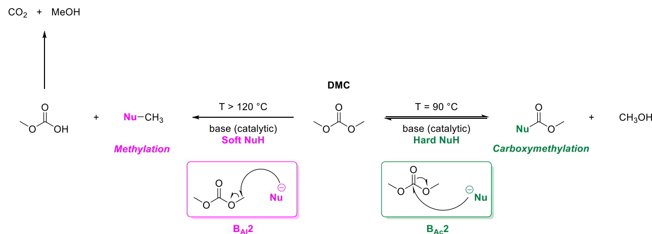
Scheme 7. DMC reactivity.
