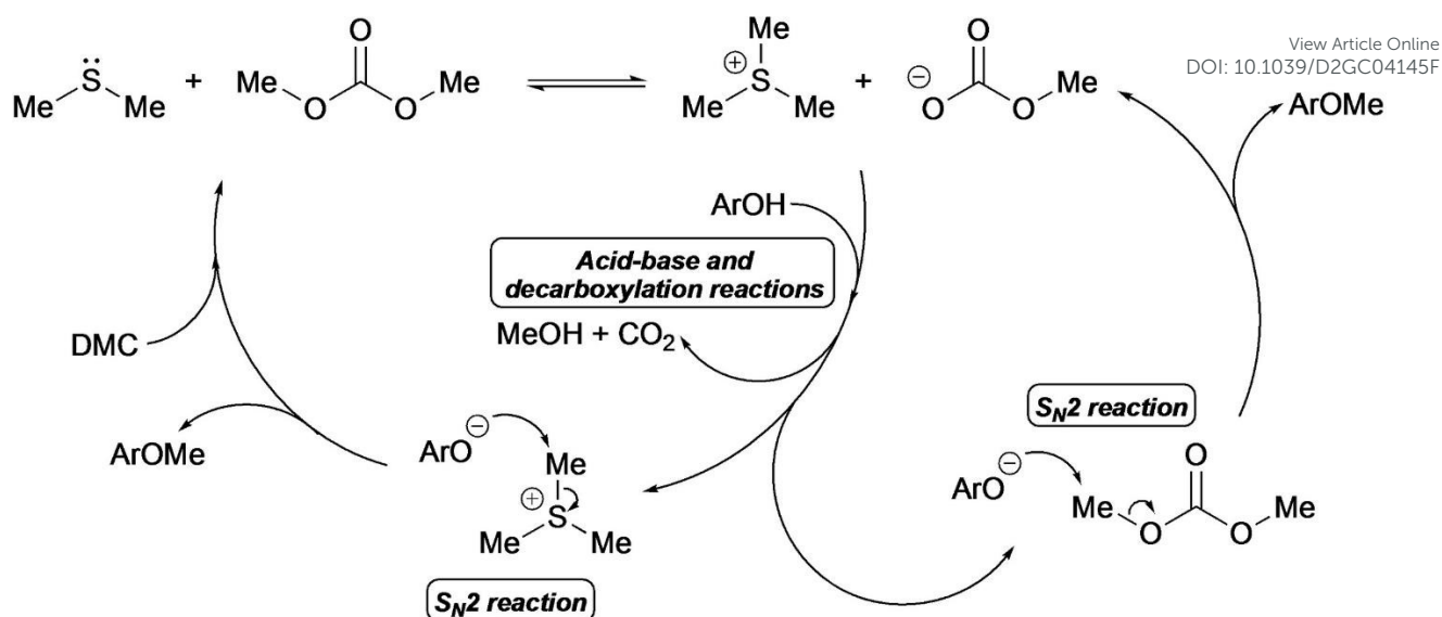
Scheme 9. Proposed mechanistic pathway for phenol methylation with DMC/Me 2 S. Reproduced with permission from ref. 98. Copyright 2022 Wiley-VCH.
