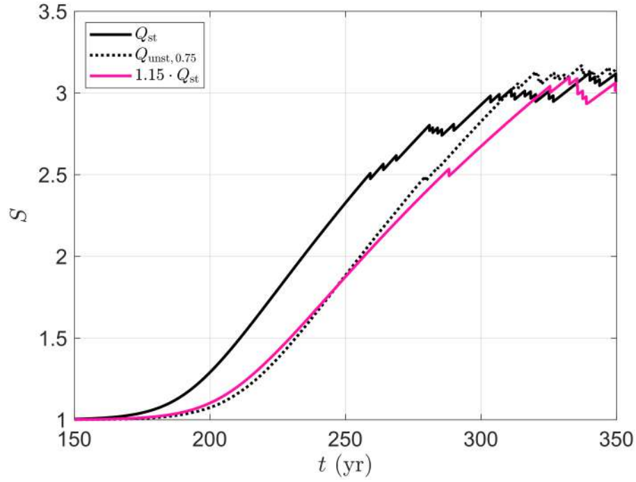
Figure S2. Temporal evolution of the sinuosity S (HIPS model) with: a steady discharge Q_{st} (black continuous line), varying flows Q_{unst} characterized by a coefficient of variation equal to 0.75 (black dotted line), and a steady discharge equal to 1.15 \cdot Q_{st} (magenta line), i.e., 15% higher than Q_{st} .
