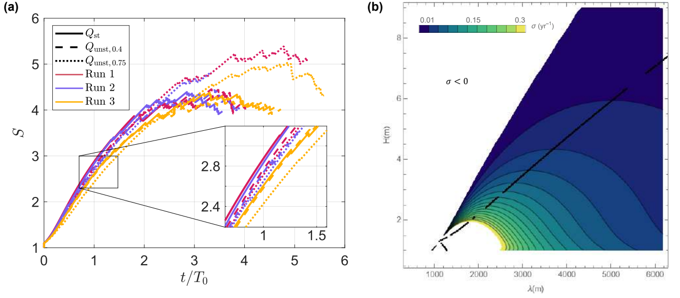
Figure S1. Numerical and theoretical results obtained with the Zolezzi and Seminara (2001) model. (a) Time series of the river sinuosity S . The colors code the three simulated rivers set. The continuous lines indicate the reference simulations forced by a steady discharge Q_{st} ; the simulations with varying discharges ( Q_{unst} ) characterized by coefficients of variation equal to 0.4 and 0.75 are represented by the dashed and dotted lines, respectively. (b) Linear analysis: contour plot of the linear growth rate \sigma obtained for the ZS model, as a function of the meander wavelength ( \lambda ) and flow depth ( H ). The black line marks the fastest-growing wavelength for any given water depth.
