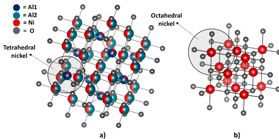
Fig. 5. a) \text{NiAl}_2\text{O}_4 structure; b) \text{NiO} (bunsenite) structure. Images elaborated with VESTA program [38].
