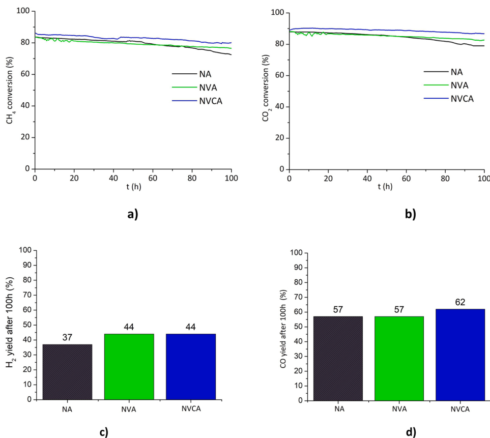
Fig. 7. Activity of the catalysts prepared, a) CH 4 conversions; b) CO 2 conversions; histograms after 100 h of reaction of c) H 2 yields and d) CO yields. Reaction conditions: 650 °C, GHSV 12000 h -1 , reagents ratio (CH 4 :CO 2 :He) 1:1:18.
