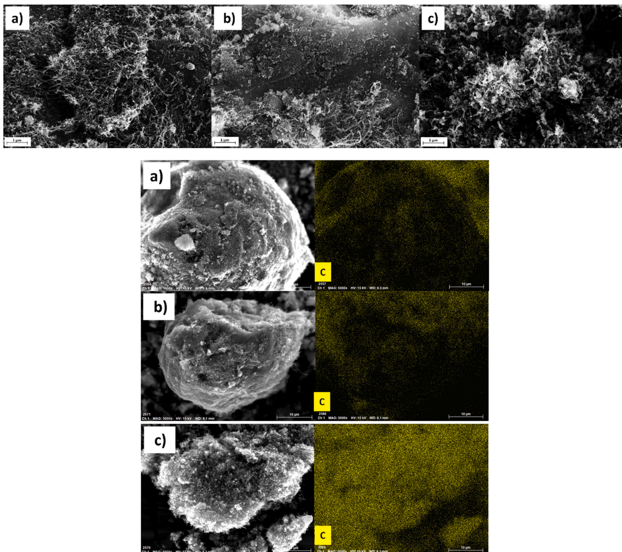
Fig. 12. SEM-EDX images of NA (a), NVA (b), NVCA (c) spent catalysts after stress tests.
