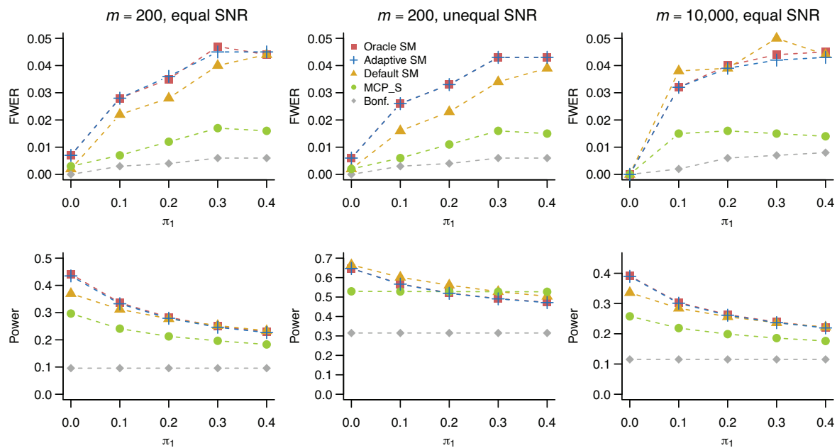
FIGURE 3 Estimated familywise error rate (first row) and power (second row) as a function of \pi_1 based on 1000 simulated data sets. The proportion of false union hypotheses is \pi_2 = 0.05 . In columns 1 and 2: m = 200 , in column 3 m = 10,000 . Signal-to-noise ratio (SNR) is 3 for all false component hypotheses in column 1; 3 for H_{11} and 6 for H_{12} in column 2, 4 in column 3. Methods are ScreenMin with the oracle threshold (square), the adaptive threshold (cross), and the default threshold (triangle); the method of Sampson et al. (2018) (circle) and the classical Bonferroni (diamond). Monte Carlo standard errors of the estimates of power and familywise error rate are 1.6 \times 10^{-2} and 7 \times 10^{-3} , respectively
