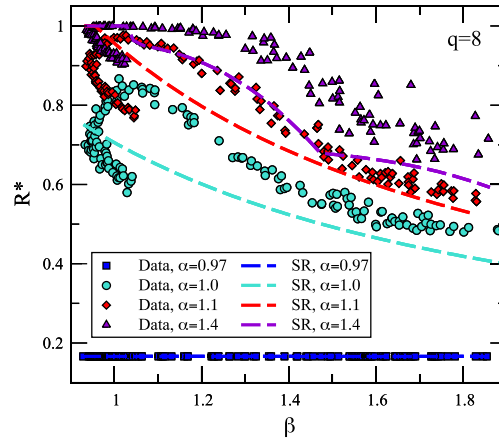
Fig. 5. Dimensional reduction of DebtRank dynamics on power-law networks (BA), for varying \beta . Plots show the steady states of the reduced variable R^* as a function of the heterogeneity \beta of the network, for different values of the control parameter \alpha . Networks have been generated using Eq. (31), tuning the exponent \nu \in [0, 2.5] . Cloud of points: results of the full DebtRank dynamics. Dashed and dotted lines: solutions of the SR and DWR, respectively, with p(h) = h^8 .
