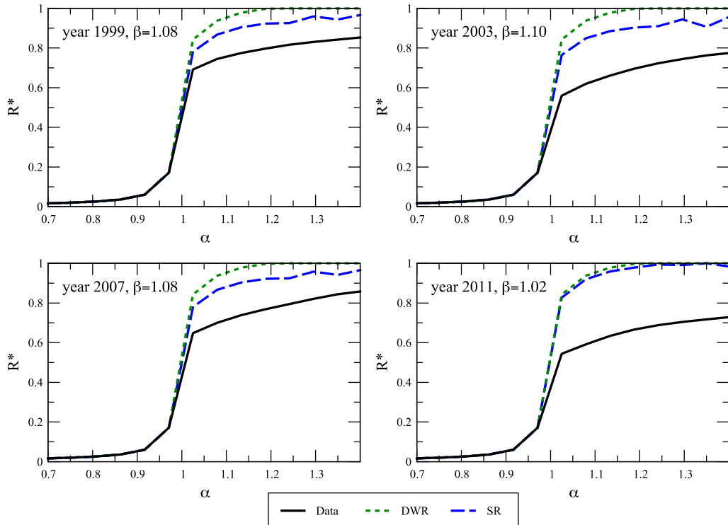
Fig. 6. Dimensional reduction of DebtRank dynamics on empirical e-MID networks. Plots show the steady states of the reduced variable R^* as a function of the spectral radius of the leverage matrix, for e-MID network data in various representative years.
