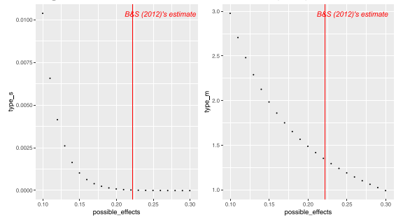
Panel (a) Type S Error Panel (b) Type M Error Figure A4.6 Table2 coefficient: Q1vsQ1Q2Female
