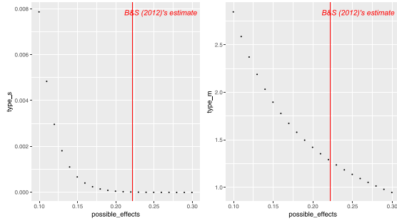
Panel (a) Type S Error Panel (b) Type M Error Figure A4.1 Table2 coefficient: NQvsQ1Male
