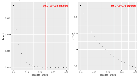
Panel (a) Type S Error Panel (b) Type M Error Figure A4.7 Table2 coefficient: Q1vsQ2Male
