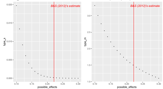
Panel (a) Type S Error Panel (b) Type M Error Figure A4.4 Table2 coefficient: NQvsQ2Female
