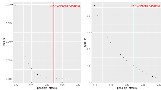
Panel (a) Type S Error Panel (b) Type M Error Figure A4.5 Table2 coefficient: NQvsQ2Female
