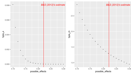
Panel (a) Type S Error Panel (b) Type M Error Figure A4.3 Table2 coefficient: NQvsQ1Q2Male
