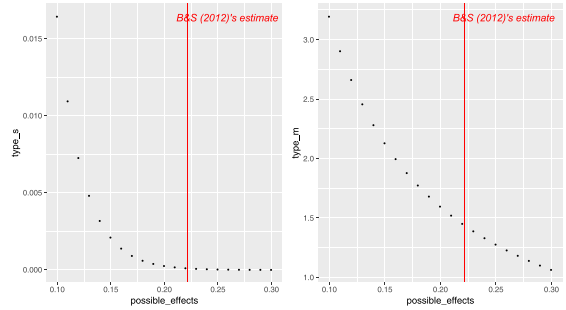
Panel (a) Type S Error Panel (b) Type M Error Figure A4.2 Table2 coefficient: NQvsQ1Q2Female
