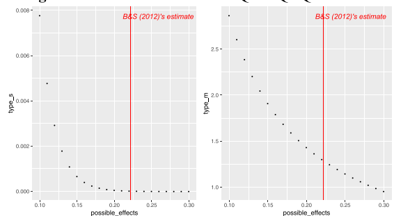
Panel (a) Type S Error Panel (b) Type M Error Figure A4.8 Table2 coefficient: Q2vsQ1Q2Male
