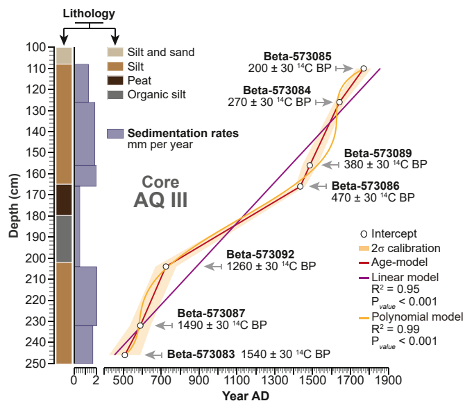
Fig. 2. Focus on the core AQ III and the radiocarbon chronology. The lithology of the core is detailed according to depth. The sedimentation rates are shown in mm per year. The radiocarbon dates are depicted as intercepts and 2-sigma calibrations (95% of probability). The age model is compared and contrasted with linear (purple line) and polynomial (orange line) regressions. (For interpretation of the references to colour in this figure legend, the reader is referred to the Web version of this article.)
