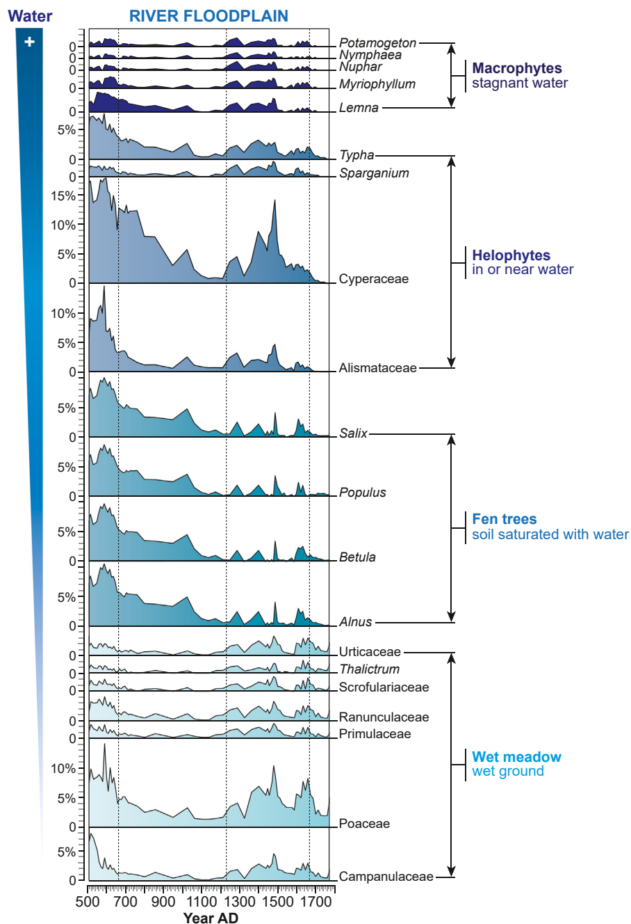
Fig. 4. Detailed pollen diagram of the Aquileia river floodplain for the period 500–1800 AD. The taxa are grouped into PdVs and plotted on a linear age-scale. The vertical lines indicate the main transitions.
