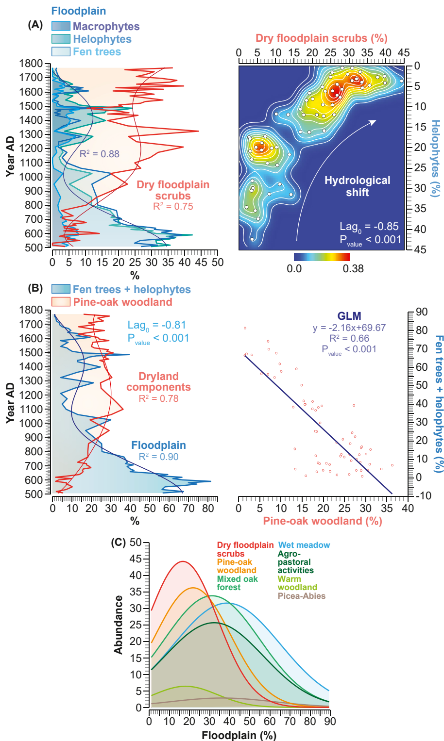
Fig. 7. Floodplain dynamics compared and contrasted with dry components. (A) Variations in the floodplain contrasted with the dynamics of the dry floodplain scrubs based on a synthetic diagram and a 2D Kernel-density model. The R^2 of the cross-correlation is indicated on the Kernel graph (B) Floodplain dynamic compared to the dryland components based on a synthetic diagram and a Generalized Linear Model. The R^2 of the cross-correlation is indicated on the synthetic diagram (C) Gradient Species packing test showing the distribution of each cluster taking the floodplain as a stationary reference. All the long-term trends are highlighted by polynomial models (order 5, P_{value} < 0.001 ).
