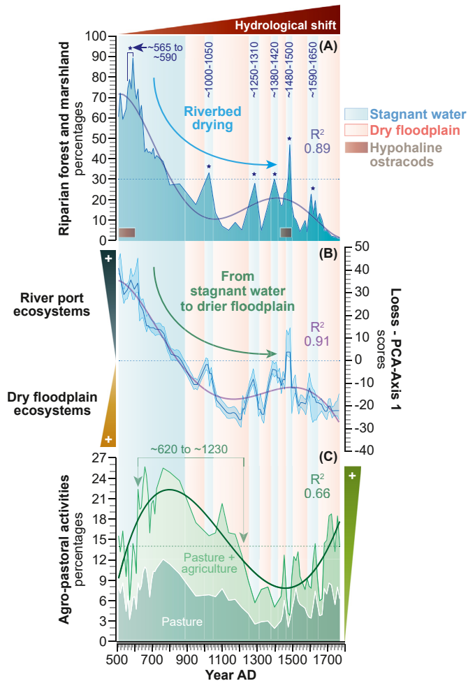
Fig. 6. Environmental dynamics of the floodplain. (A) Evolution of the floodplain depicted by the riparian forest and marshland. The occurrence of hypohaline ostracods is also shown. (B) Loess PCA-Axis 1 (77% of total variance) shown with the 95% confidence band. (C) Pastoral activities alone (dark green) and pastoral activities with agriculture (light green) are plotted on a linear age-scale. All the long-term trends are highlighted by polynomial models (order 5, P_{\text{value}} < 0.001 ). (For interpretation of the references to colour in this figure legend, the reader is referred to the Web version of this article.)
