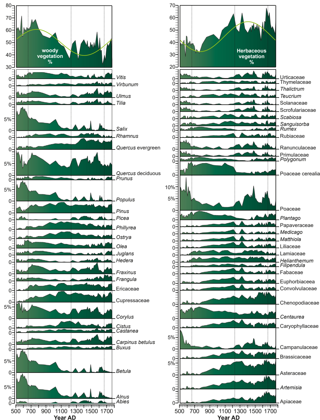
Fig. 3. Detailed pollen diagram (woody and herbaceous vegetation) for the period 500–1800 AD. The taxa are plotted on a linear age-scale. The vertical lines indicate the main transitions.
