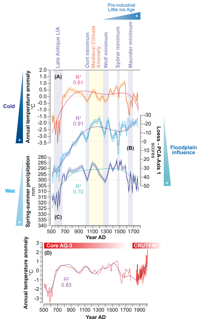
Fig. 9. Pollen-based climate reconstruction. (A) Temperature anomalies (with the standard deviations) plotted on a linear age-scale. (B) Loess PCA-Axis 1 (77% of the total variance) shown with the 95% confidence band. (C) Spring-summer precipitation (with the standard deviations) plotted on a linear age-scale. All the long-term trends are depicted by polynomial models (order 5, P_{value} < 0.001 ). (D) Temperature anomalies compared and contrasted with the 1850–2019 CRUTEM4 data (Osborn and Jones, 2014). The sinusoidal model ( P_{value} < 0.001 ) is depicted as a purple line. (For interpretation of the references to colour in this figure legend, the reader is referred to the Web version of this article.)
