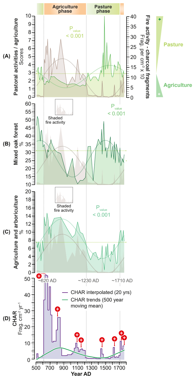
Fig. 8. Agriculture, pasture and fire activity. (A) Ratio pasture activities/agriculture and fire dynamics plotted on a linear age-scale. (B) Mixed oak forest dynamics compared and contrasted with fire activity (shown as a shaded curve). (C) Agropastoral activities contrasted with the fire activity (shown as a shaded curve). (D) CHAR analysis plotted on a linear age-scale. The red circles with white crosses denote the fire episodes. All the long-term trends are depicted by polynomial models (order 5, P_{value} < 0.001 ). (For interpretation of the references to colour in this figure legend, the reader is referred to the Web version of this article.)
