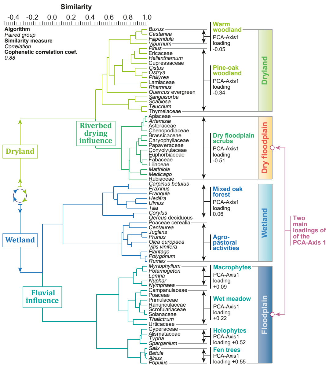
Fig. 5. Pollen-based ecological clusters from Aquileia for the period 500–1800 AD. A cluster analysis (Paired group as algorithm, Correlation as similarity measure) was used to define the ecological assemblages. Each cluster was summed to create the PdVs. The PCA loadings of each PdV are indicated on the graph.
