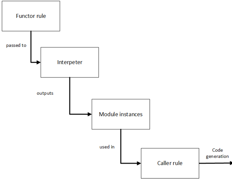
Figure 5.2: Functor processing
