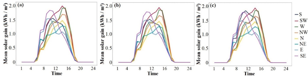
Fig. 16. Hourly solar gain ( \text{kWh/m}^2 ) under different orientation during (a) Present TMY; (b) 2050; and (c) 2080.
