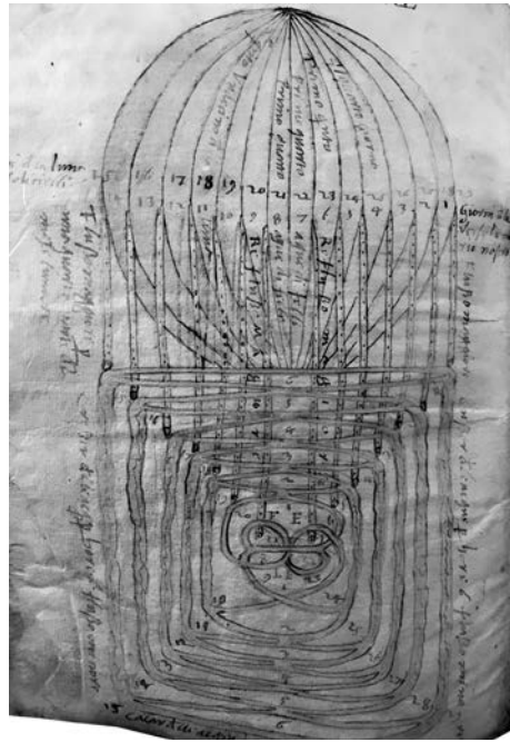
Fig. 5: A graph illustrating the correlation among different phases of the lunar cycle and the intensity of tidal motion.
