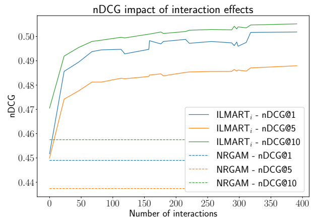
Figure 2: Initial analysis of interpretability effectiveness tradeoff presented in ILMART [11] analyzing the impact of the number of interaction effects used by the model.
