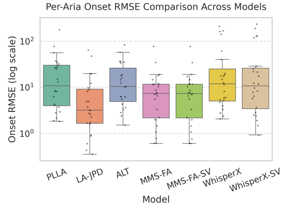
Figure 2: RMSE values across models for the 24 arias. The y-axis uses a log scale due to large performance variations across arias.
