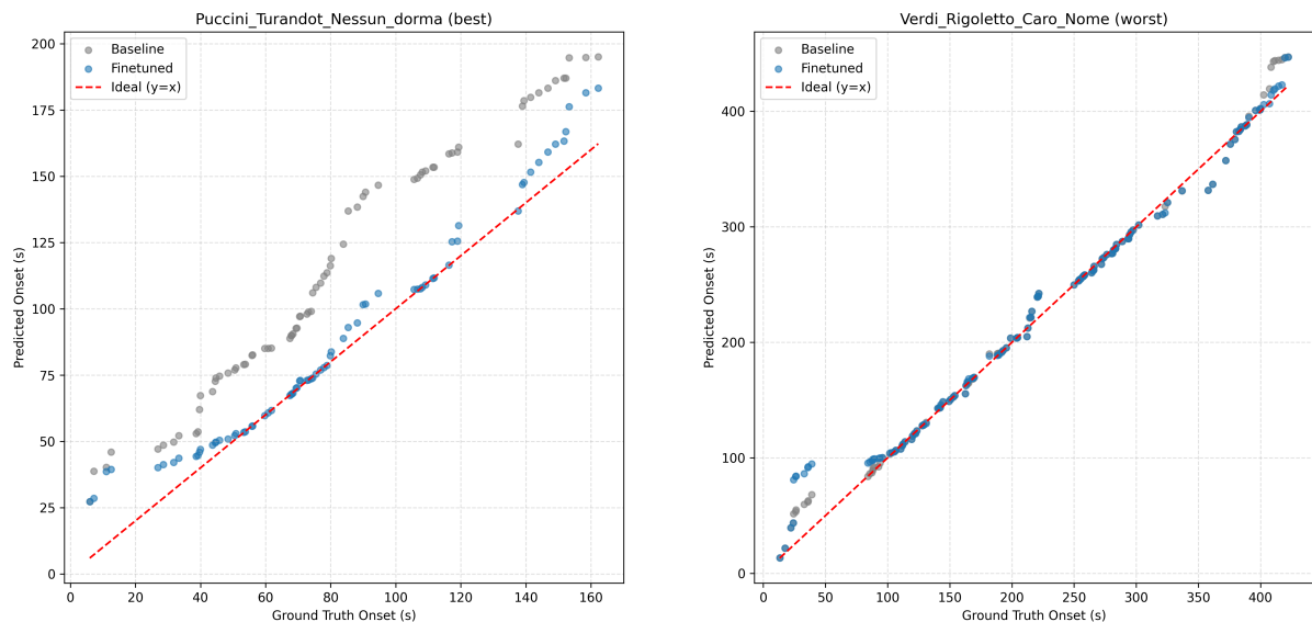
(a) Best improvement: Puccini Turandot Nessun Dorma
