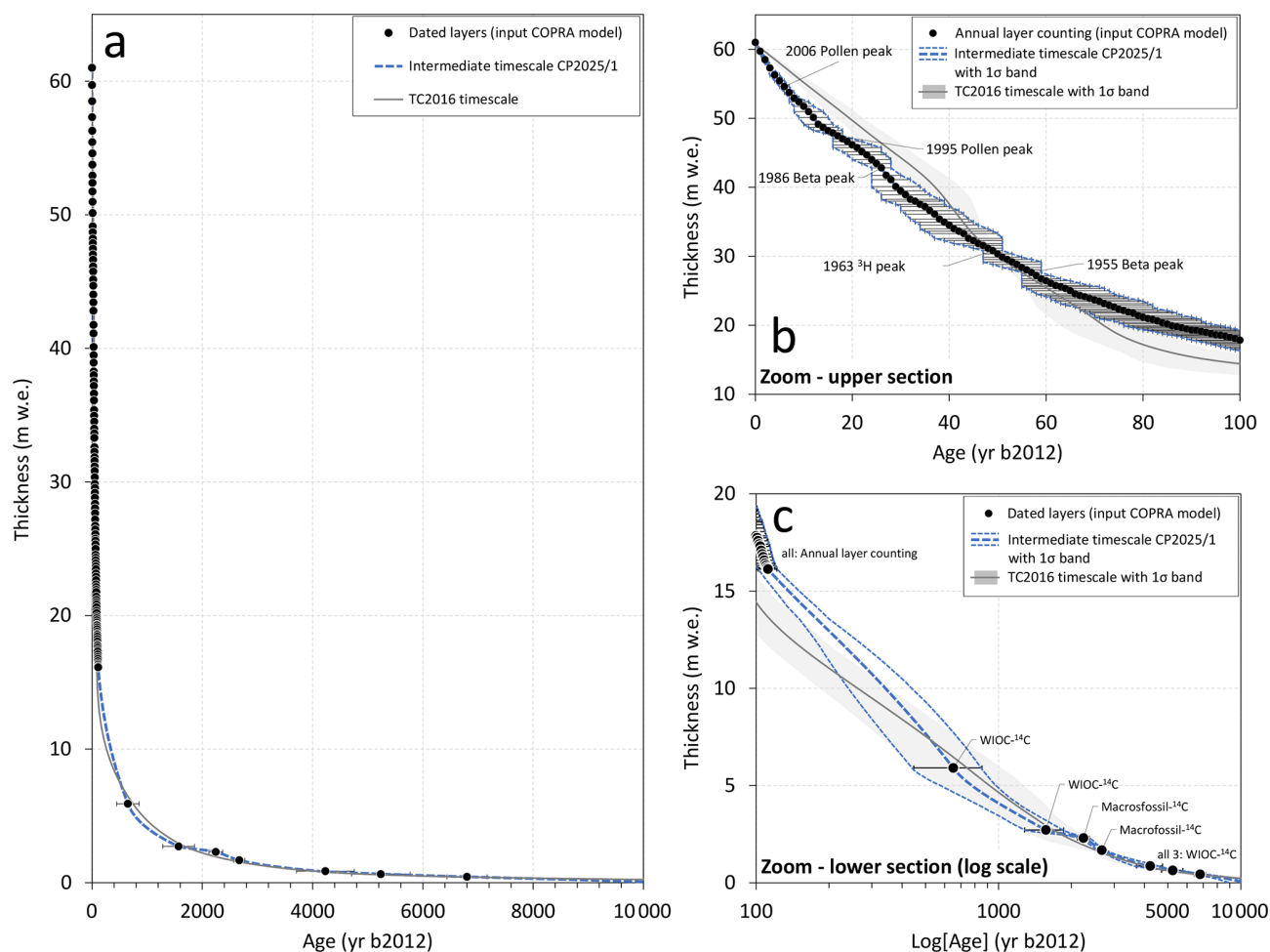
Figure 5. Comparison of the TC2016 and the updated, intermediate Alto dell'Orties (CP2025/1) timescales obtained by using COPRA. The different time markers for construction (see Table S2) are indicated by symbols with error bars representing their uncertainty by the linked dating methods ( 1\sigma range for ^{14}\text{C} cal ages; see text for others). Shown in panel (a) for the entire length of the ice core from surface, indicated by the uppermost point, to bedrock covering the entire period of the Alto dell'Orties ice archive, in panel (b) for the last 100 years, and in panel (c) for the older part of the record ( > 100 years) on a logarithmic age scale. The core #2 reference depth (Sect. 2) is here expressed as thickness, with the surface of depth zero corresponding to the total of 61.15 m w.e. (74.88 m).
