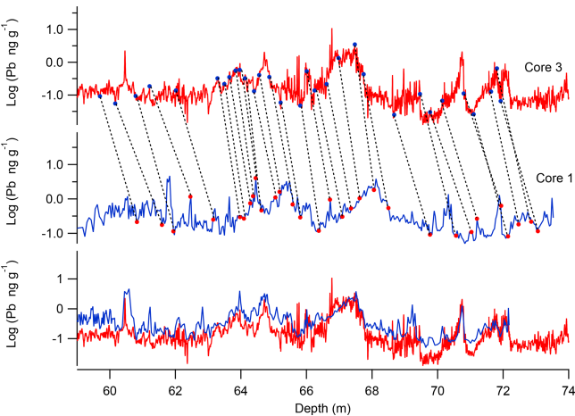
Figure 2. Pb concentrations in the deep portion of cores #3 (red; Continuous Flow Analysis ICP-SFMS, the Ohio State University) and #1 (blue; discrete ICP-MS analysis, University of Venice) at their respective #1 and #3 depth scales (upper two panels) and matched to core #3 depth (lower panel).
