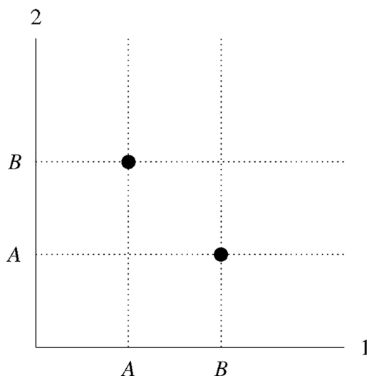
Figure 2. Configuration space representation of a two-particle world.
