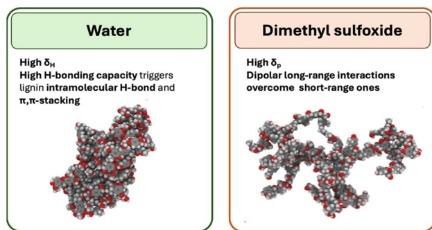
Fig. 10 A molecular simulation of lignin conformation in water and DMSO, respectively, has been reported. 93 The high hydrogen-bonding parameter ( d_{\text{H}} ) of water, indicative of strong short-range hydrogen bonding, enhances intramolecular \pi – \pi stacking and hydrogen bonds within lignin, thereby promoting a collapsed molecular configuration. In contrast, the high polarity parameter ( d_{\text{p}} ) of DMSO facilitates extended dipolar interactions between lignin and the solvent, favoring an elongated conformation. Reproduced from ref. 72 with permission from Nature, copyright 2024.
