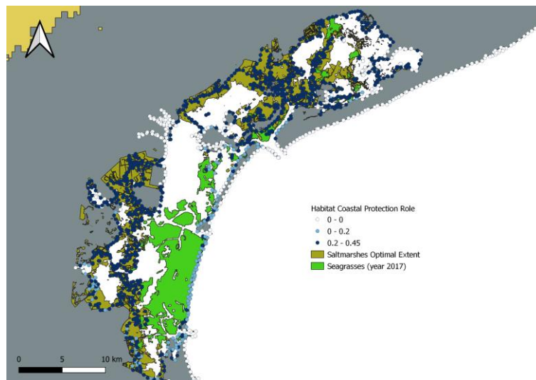
SI.5: Habitat coastal protection role Scenario No SLR - Augmented Seagrass Habitat and Current Saltmarsh Habitat
