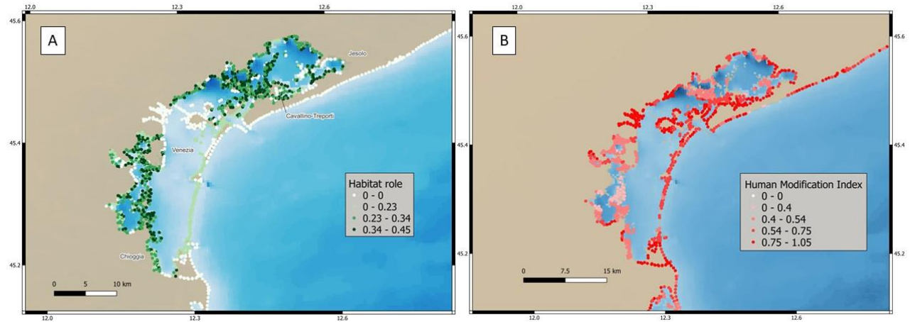
Figure 9: A) Habitat Role map. The habitat role is a measure of the protection offered by the habitats, it is calculated as the difference between the Exposure Index including seagrasses and salt marshes and the Exposure Index without those habitats for each 250 m coastline segment for the entire study area. The role of habitats is a relative measure of how mangroves reduce exposure to coastal flooding and erosion. B) Human Modification Index map.
