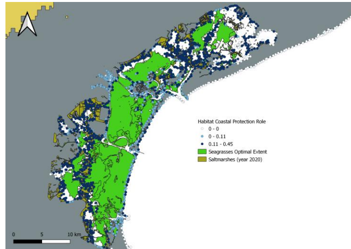
SI.6: Habitat coastal protection role Scenario No SLR - Augmented Seagrass Habitat and Augmented Saltmarsh Habitat
