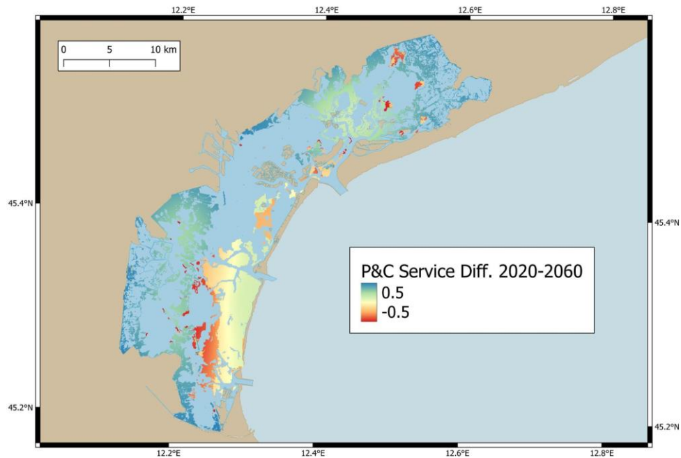
Figure 11: The difference between the P&C Index in the year 2020 and the year 2060. The total sum of pixels is equal to -9130 and the mean value is -0.004, indicating a general decrease in the P&R index across the lagoon, even with a small disturbance.
