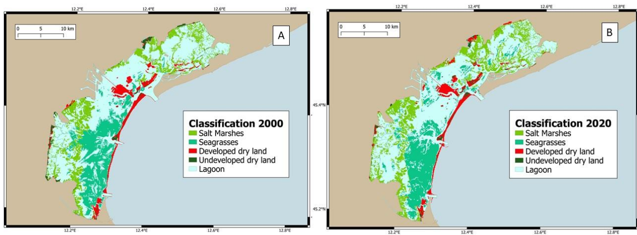
Figure 6: Land use classification performed with the Semi-Automatic Classifier in QGIS for the years A) 2000 and, B) 2020.
