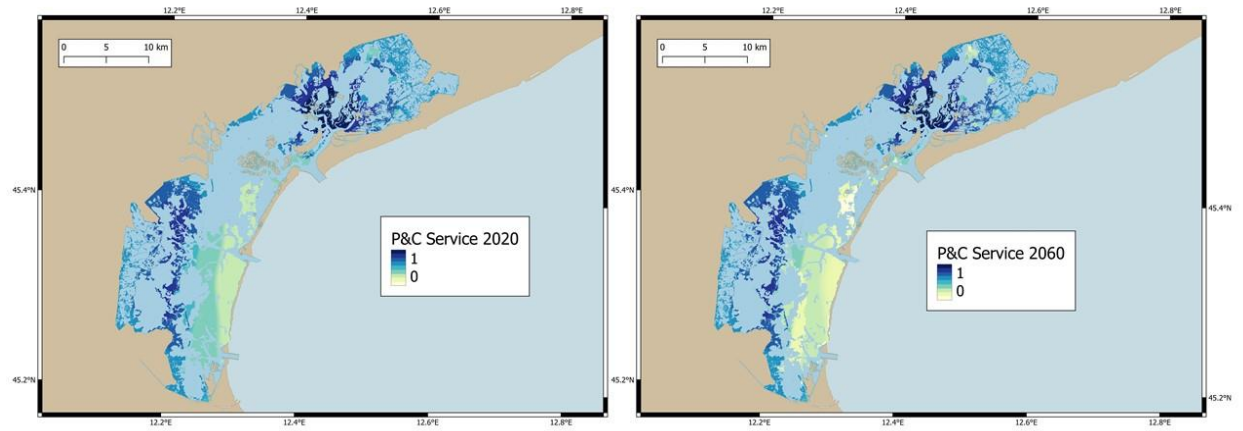
Figure 10: The P&C Index Map for the years 2020, which is the beginning of the studied period and 2060, which is the last year of the study.
