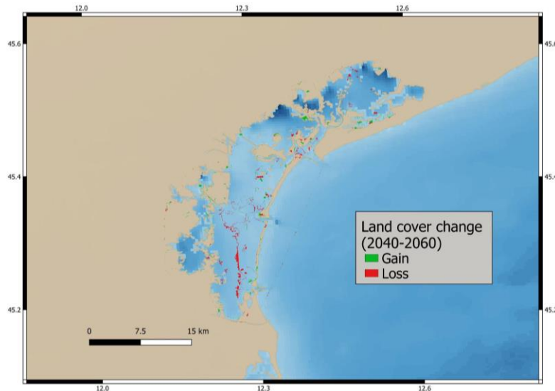
Figure 7: Gain and loss extension between the two simulated layers in Molusce for the projected years 2040 and 2060.
