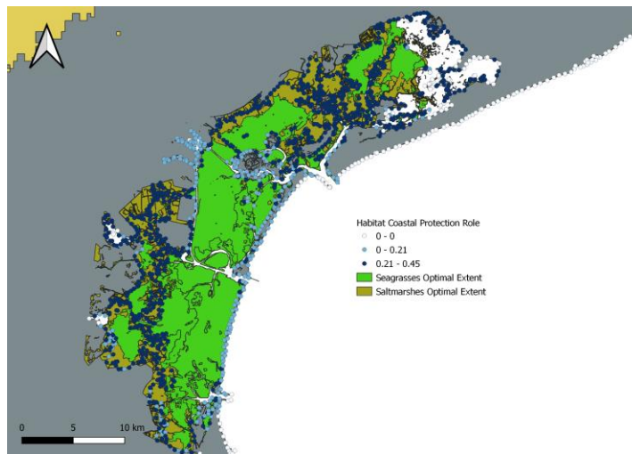
SI.7: Habitat coastal protection role Scenario RSLR 4.5 year 2050 - Current Habitats
