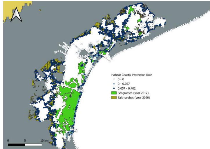
SI.8: Habitat coastal protection role Scenario RSLR 4.5 year 2050 - Current Seagrass Habitat and Augmented Saltmarsh Habitat
