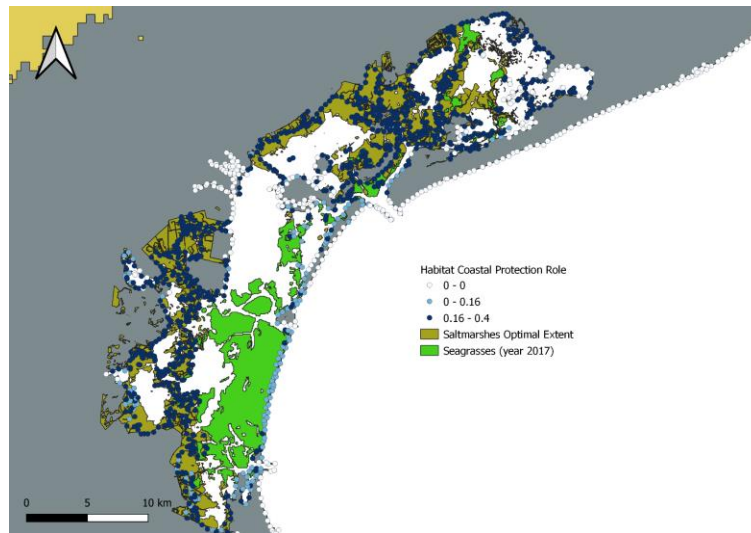
SI.9: Habitat coastal protection role Scenario RSLR 4.5 year 2050 - Augmented Seagrass Habitat and Current Saltmarsh Habitat
