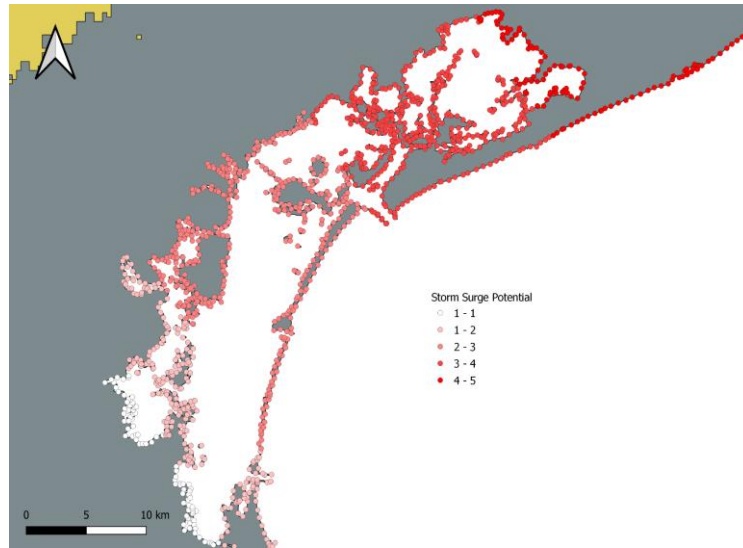
Figure 11: Relative risk of exposure to storm surge for the Venice Lagoon Coastal Areas.
