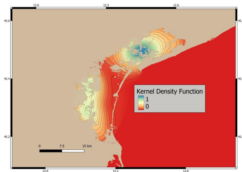
Figure 8: Normalized Kernel Density Function of the Habitat Role Index.
