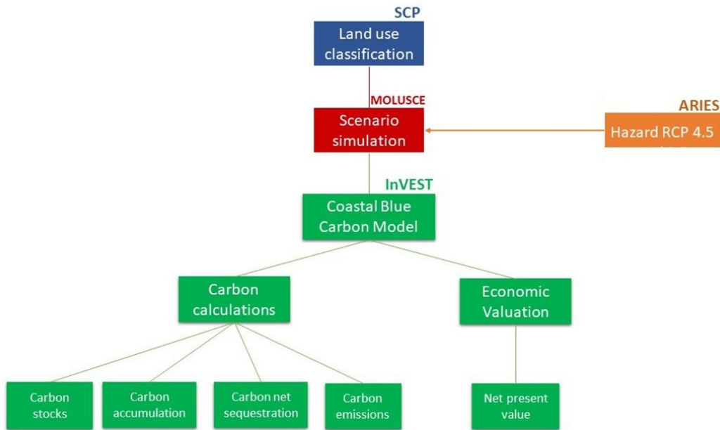
Figure 5: Diagram of the processes, softwares and outputs we follow to run the Coastal Blue Carbon Model.
