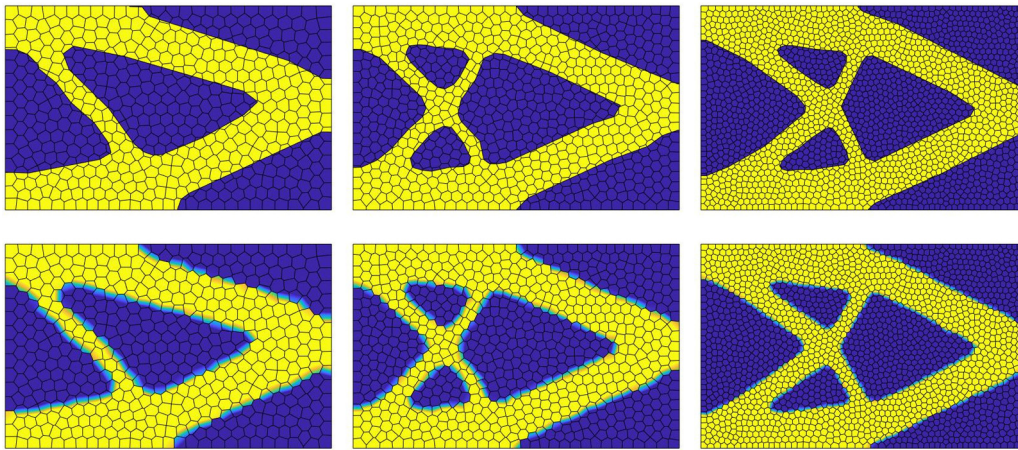
Fig. 7. Test case of Section 3.4.1 - Indicator function \chi_{\varphi,h}^{k,cl} superimposed to the mesh for a level set-fitted (top) and a non-fitted (bottom) approach, for a different cardinality \#\mathcal{T}_h^{ls} of the level set grid (from left to right, \#\mathcal{T}_h^{ls} = 500, 750, 2000 ).
