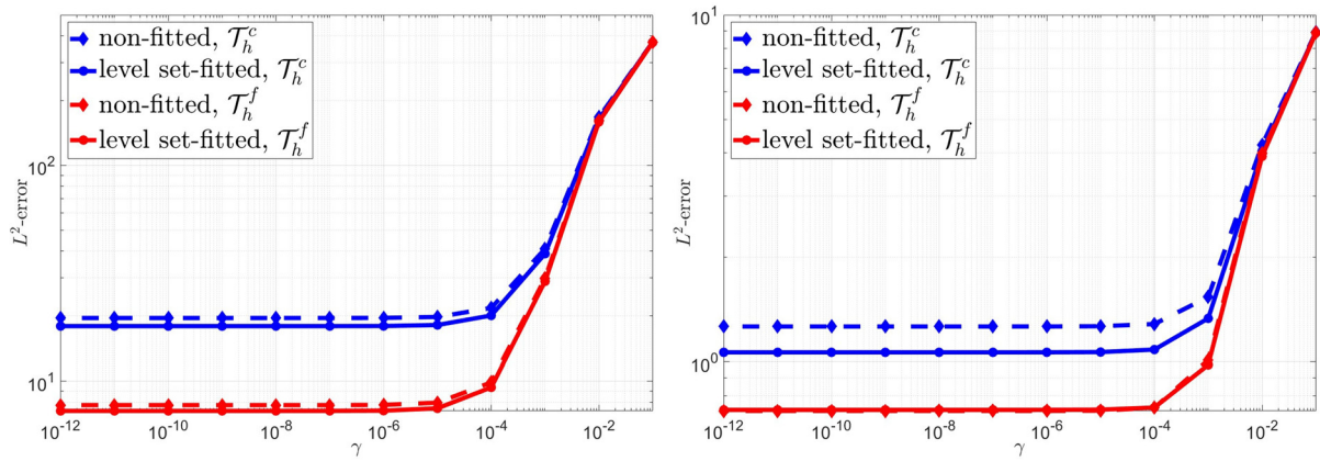
Fig. 3. Test case of Section 2.2.1 - Computed L^2(\Omega_1) -error associated with the displacement field (left) and the von Mises stress (right) for meshes \mathcal{T}_{h,j}^c and \mathcal{T}_{h,j}^f , with j = 2 (non-fitted) and j = 3 (level set-fitted), as a function of \gamma .
