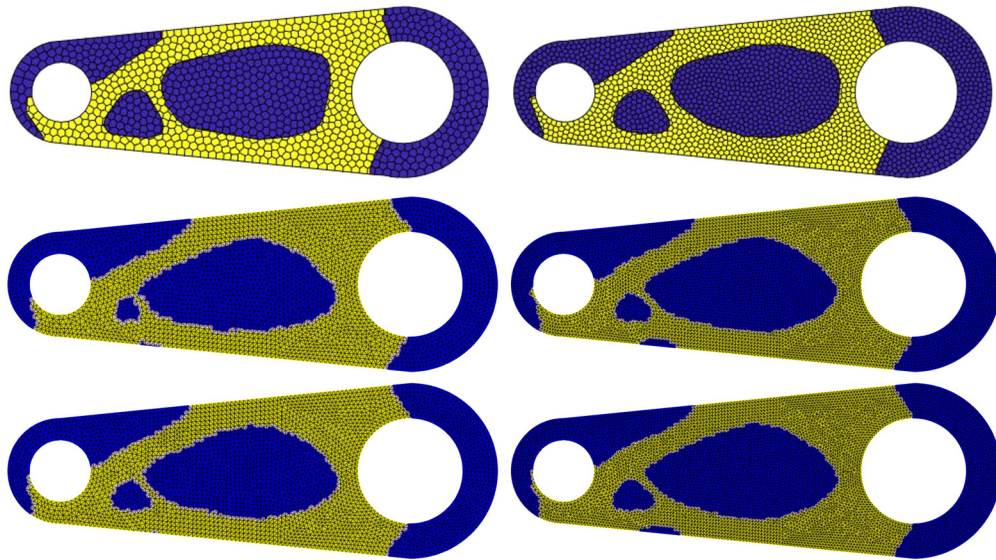
Fig. 12. Test case of Section 3.4.3 - Indicator function \chi_{\varphi,h}^{k,el} superimposed to the level set-fitted mesh, for \#\mathcal{T}_h^{ls} = 1000 (top row, left) and 2000 (top row, right); indicator function of a structure yielded by a continuous Galerkin-based topology optimization, superimposed to the unstructured triangular mesh with N_{w,ls}^c (mid row, left), N_{w,ls}^f (mid row, right), N_{w,el}^c (bottom row, left), N_{w,el}^f (bottom row, right) dofs.
