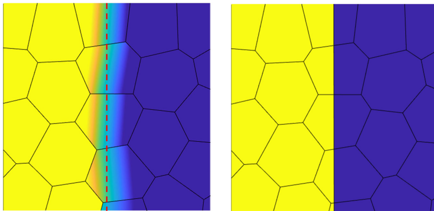
Fig. 4. Test case of Section 2.2.1 - Enlarged view of the two material-transition in correspondence with the vertical interface for the non-fitted (left) and the level set-fitted (right) mesh.
