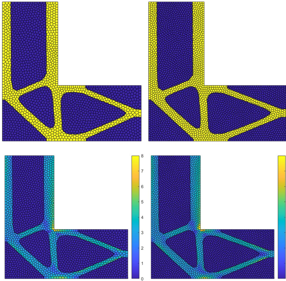
Fig. 8. Test case of Section 3.4.2 - Indicator function \chi_{\varphi,h}^{k,el} (top) and corresponding von Mises stress distribution (bottom) superimposed to the fitted mesh, for a different cardinality \#\mathcal{T}_h^{ls} of the level set grid ( \#\mathcal{T}_h^{ls} = 2000 , left; \#\mathcal{T}_h^{ls} = 3000 , right).
