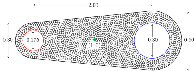
Fig. 11. Test case of Section 3.4.3 - Geometry and polygonal computational mesh with non-homogeneous Neumann (red-highlighted) and homogeneous Dirichlet (blue-highlighted) boundary portions.
