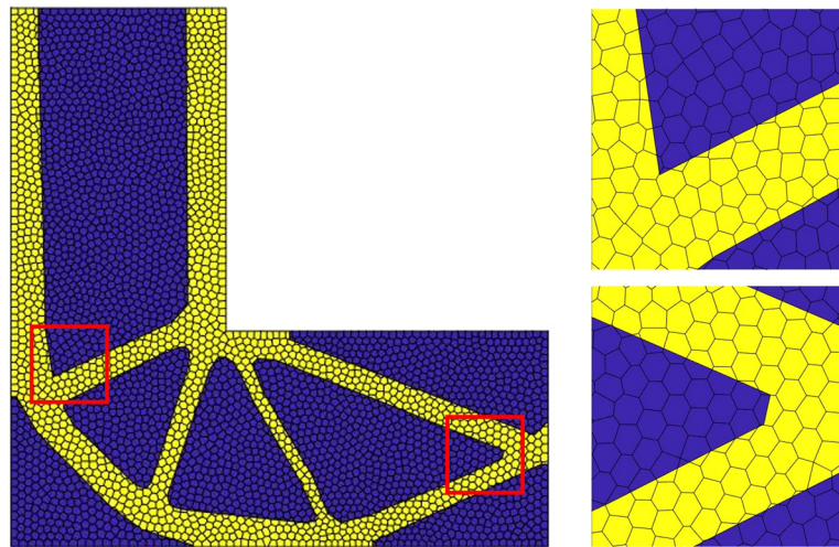
Fig. 10. Test case of Section 3.4.2 - Indicator function \chi_{\varphi,h}^{k,el} superimposed to the level set-fitted mesh (left) and enlarged views (right), for \#\mathcal{T}_h^{ls} = 3500 .
