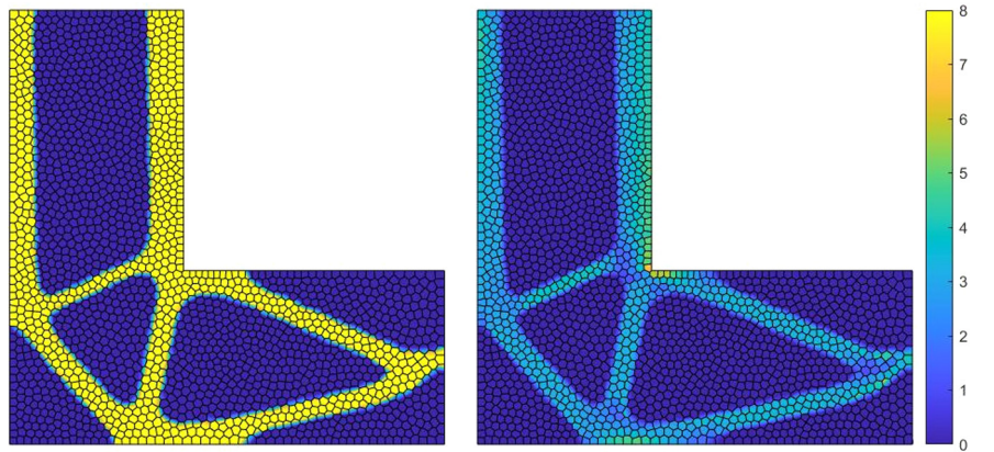
Fig. 9. Test case of Section 3.4.2 - Indicator function \chi_{\varphi,h}^{k,el} (left) and corresponding von Mises stress distribution (right) superimposed to the non-fitted mesh, for \#\mathcal{T}_h^{ls} = 2000 .
