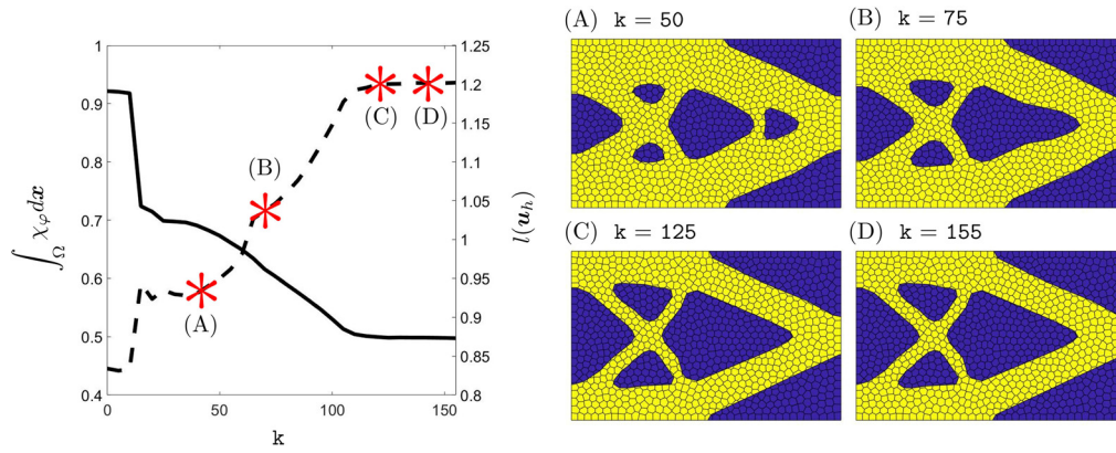
Fig. 6. Test case of Section 3.4.1 - Convergence history (left) of the compliance (dashed line) and of the volume fraction (solid line); indicator function \chi_{\varphi,h}^{k,cl} superimposed to the fitted mesh (right) at iterations k = 50, 75, 125, 155 , red-highlighted in the left panel.
