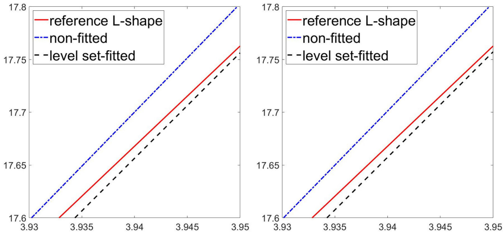
Fig. 5. Test case of Section 2.2.1 - PolyDG approximation of the vertical displacement field component along the cut line r : \{y = x, 3.93 \leq x \leq 3.95\} for scenarios i), ii), and iii), for \gamma = 1e-6 (left) and \gamma = 1e-12 (right).
