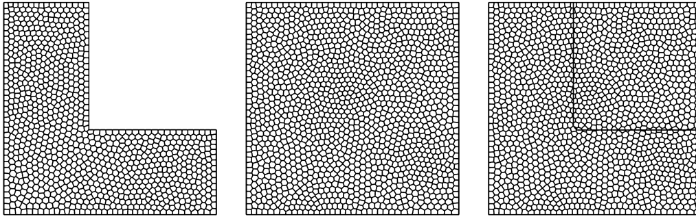
Fig. 2. Test case of Section 2.2.1 - Example of the considered meshes for test cases i) (left), ii) (center), and iii) (right).
