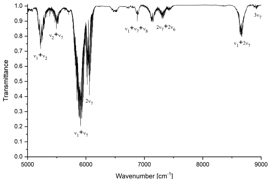
Fig. 2. Gas-phase survey spectrum of \text{CH}_2\text{DCl} in the spectral region 5000–9000 \text{cm}^{-1} . Resolution = 0.5 \text{cm}^{-1} , room temperature, optical path length = 37.5 m, P = 2.1 kPa. Only some relevant absorptions are labeled.
