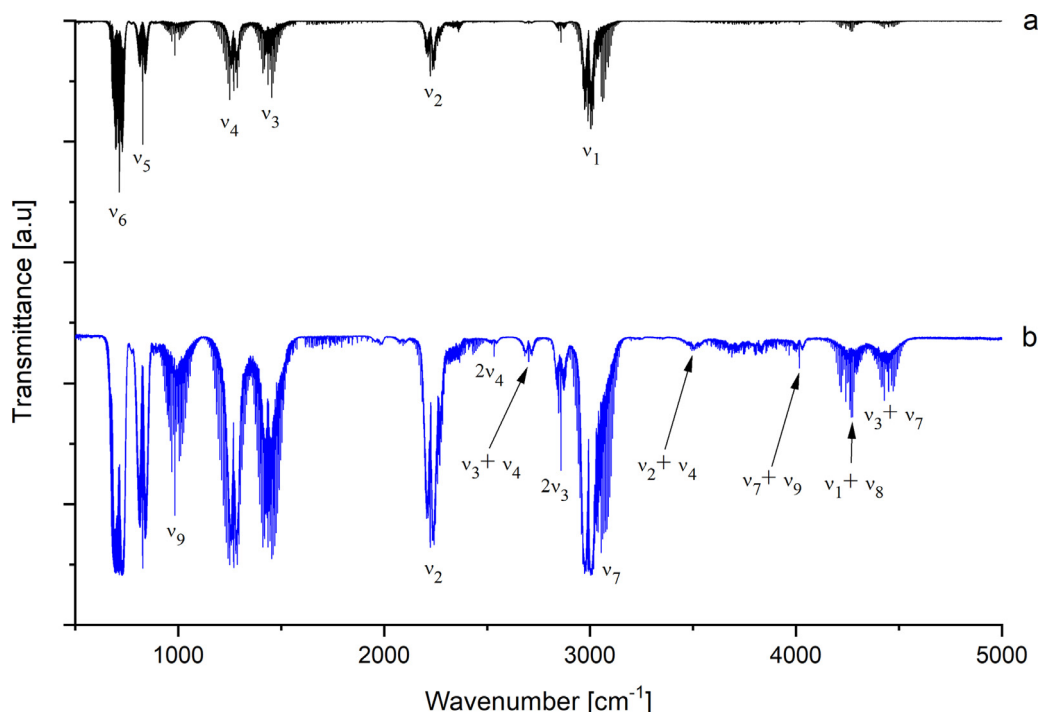
Fig. 1. Gas-phase survey spectra of \text{CH}_2\text{DCl} in the spectral region 500–5000 \text{cm}^{-1} . (a) Resolution = 0.2 \text{cm}^{-1} , room temperature, optical path length = 6 m, P = 1.7 kPa; (b) resolution = 0.5 \text{cm}^{-1} , room temperature, optical path length = 0.16 m, P = 12.5 kPa. Both traces were vertically shifted for clarity. Only some relevant absorptions are labeled.
