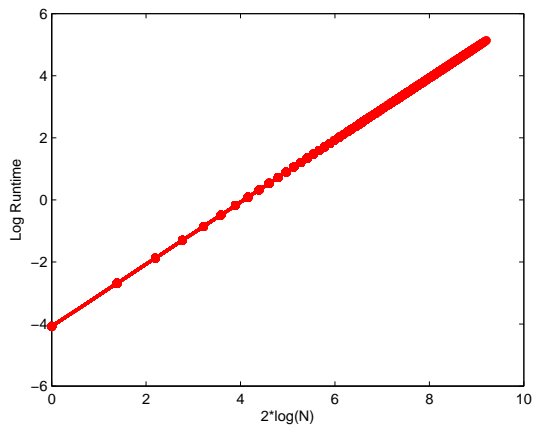
(c) Log Runtime vs 2 \log(N) using QJSA Kernel.
